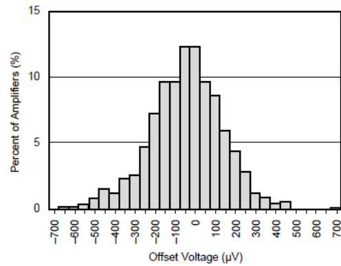
FIG 5-8. Offset Voltage Production Distribution
