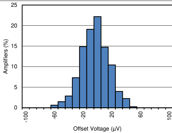
FIG 1. Input Referred Offset Voltage Distribution
