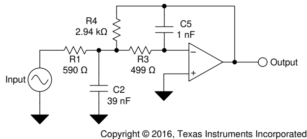
图 47. Typical OPA207 Application Schematic
