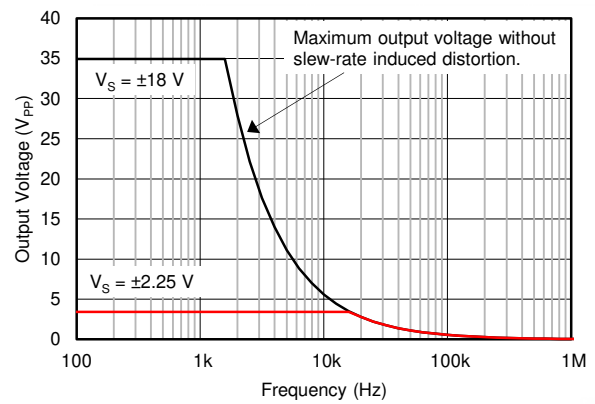
FIG 38. Maximum Output Voltage Amplitude vs Frequency
