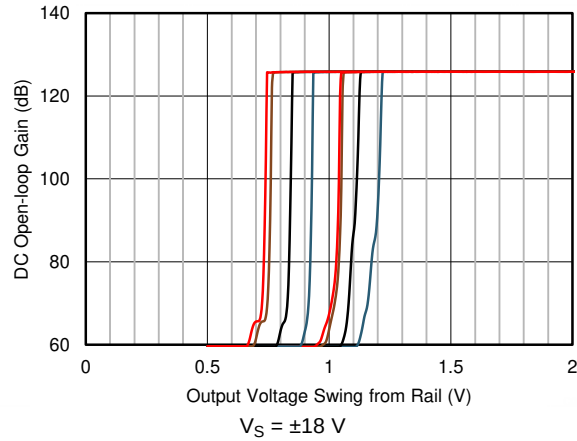
FIG 25. Open-Loop Gain vs Output Voltage Swing to Supply
