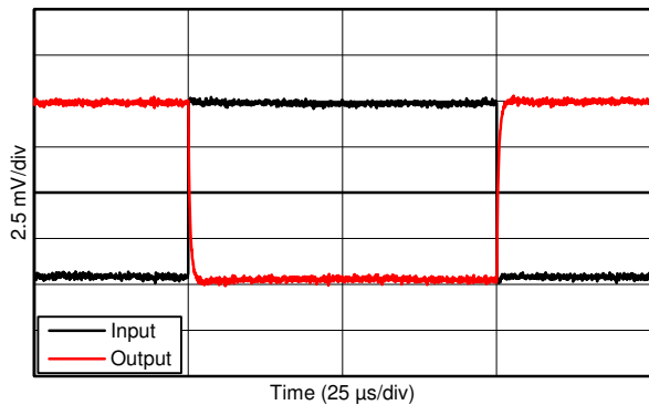
FIG 31. Negative Overload Recovery
