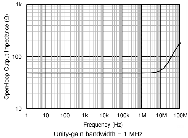
FIG 27. Open-Loop Output Impedance vs Frequency
