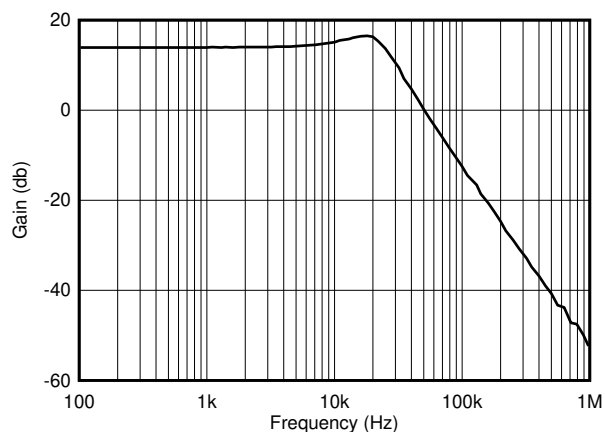
FIG 48. OPAx202 Second-Order, 25-kHz, Chebyshev, Low-Pass Filter
