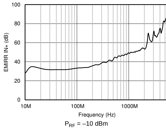
FIG 39. EMIRR vs Frequency
