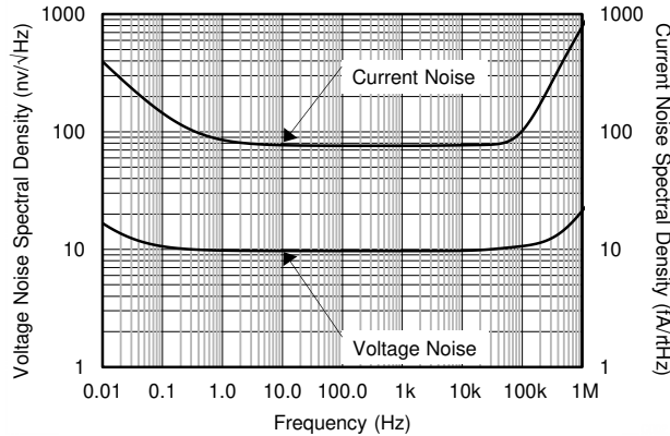
FIG 19. Input Voltage Noise Spectral Density vs Frequency
