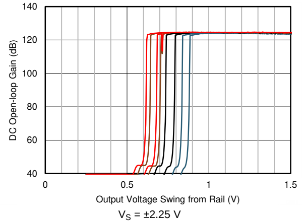
FIG 26. Open-Loop Gain vs Output Voltage Swing to Supply
