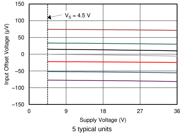
FIG 7. Offset Voltage vs Supply Voltage
