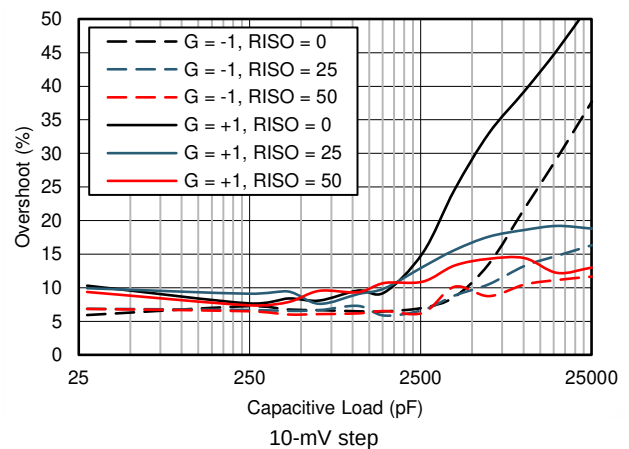
FIG 28. Small-Signal Overshoot vs Capacitive Load
