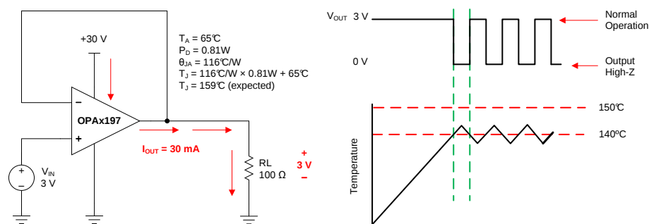
Figure 46. Thermal Protection
