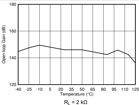
FIG 6-23. Open-Loop Gain vs Temperature
