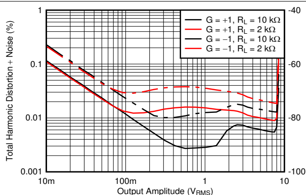
FIG 6-19. THD+N vs Output Amplitude
