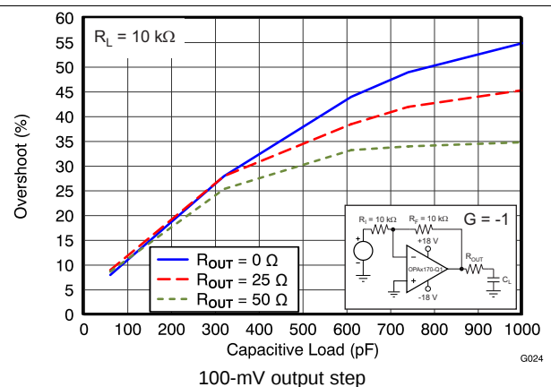
24. Small-Signal Overshoot vs Capacitive Load
