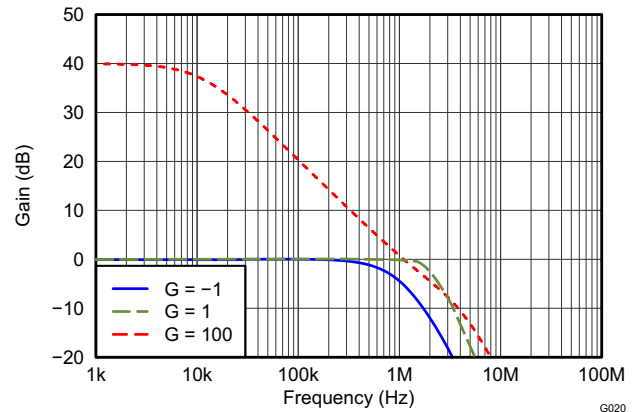
20. Closed-Loop Gain vs Frequency
