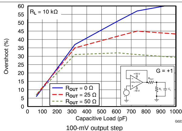
23. Small-Signal Overshoot vs Capacitive Load
