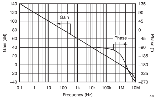
19. Open-Loop Gain and Phase vs Frequency
