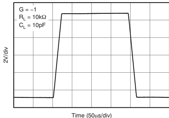
FIG 31. Large-Signal Step Response
