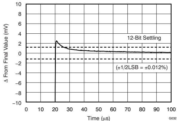
FIG 32. Large-Signal Settling Time
