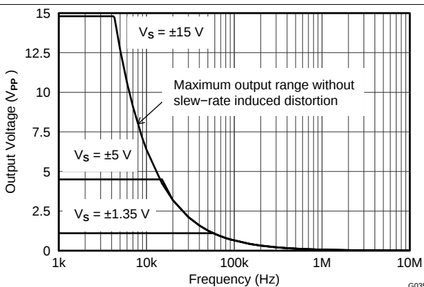
FIG 35. Maximum Output Voltage vs Frequency
