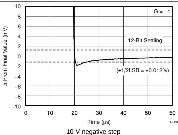
FIG 33. Large-Signal Settling Time
