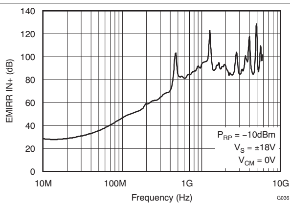
FIG 36. EMIRR IN+ vs Frequency
