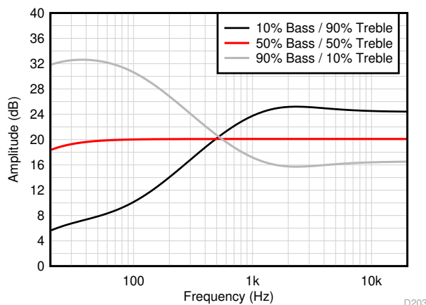
8-10. Amplitude vs Frequency for Various Tone-Control Settings
