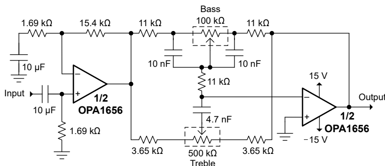
8-9. Dual Potentiometer Baxandall Tone Control
