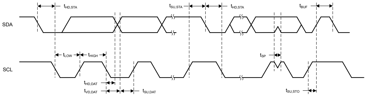
図 7-4. I2C Timing Diagram
