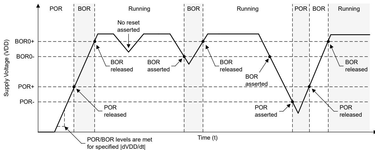
図 7-1. Power Cycle POR/BOR Conditions
