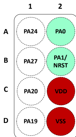
図 6-8. 8-Pin YCJ (DSBGA) (Bumps Down View)
