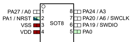
6-6. 8-Pin DDF (SOT) (Top View)
