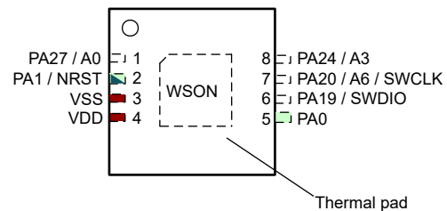
6-7. 8-Pin DSG (WSO) (Top View)
