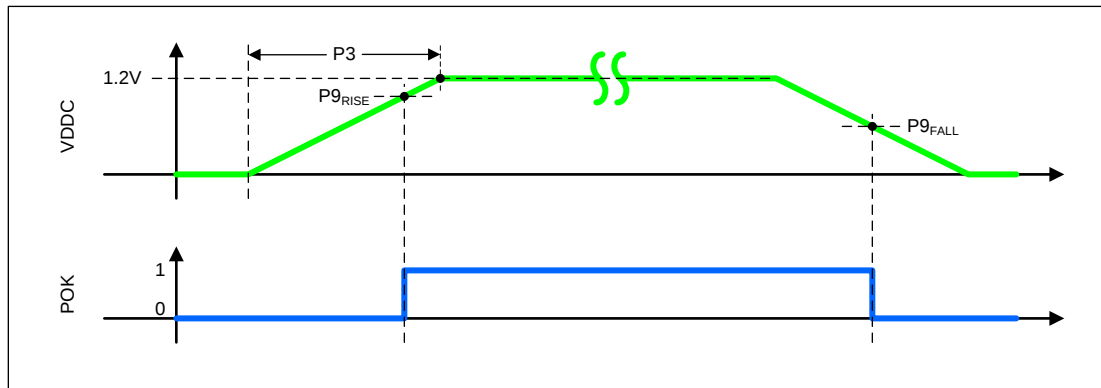
5-4. POK Assertion vs V_{DDC}
