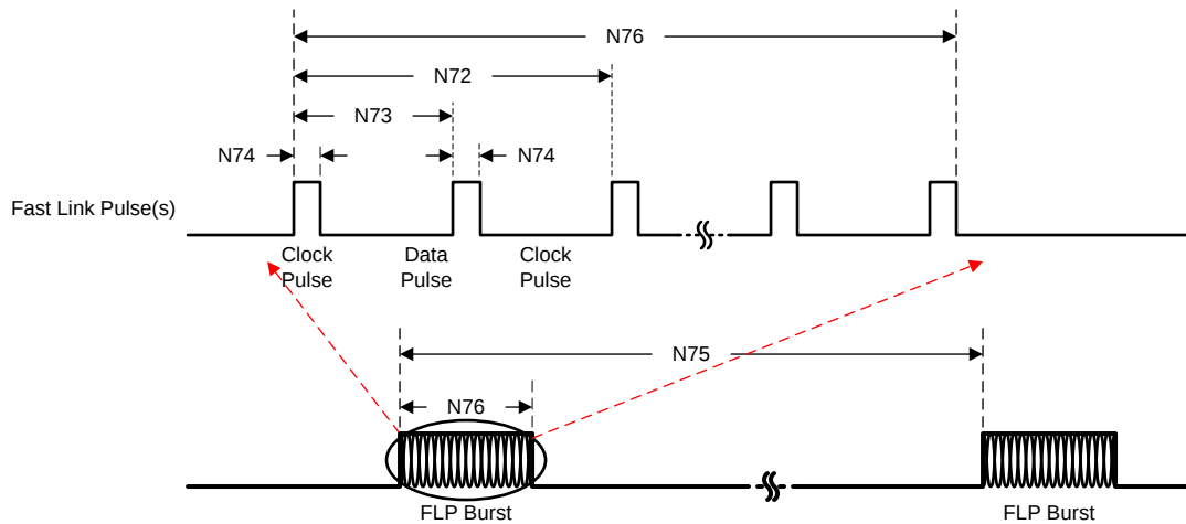
図 5-43. Auto-Negotiation Fast Link Pulse Timing
