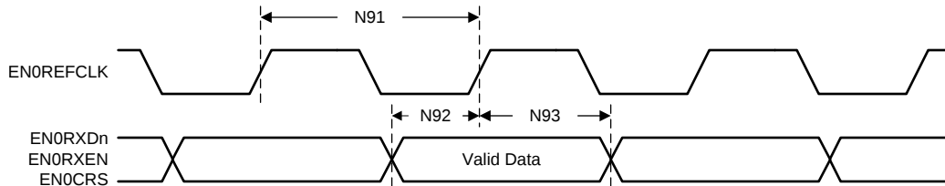
图 5-46. RMII Receive Timing
