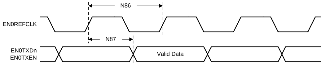
图 5-45. RMII Transmit Timing
