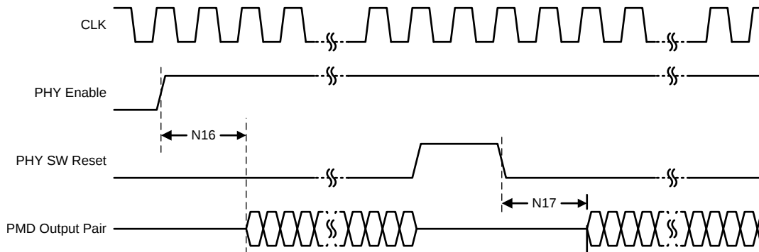
图 5-35. Reset Timing
