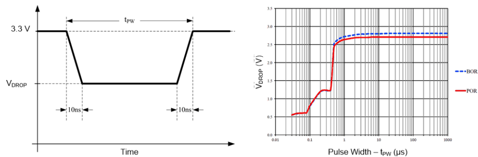
5-6. POR-BOR V_{DD} Droop Response
