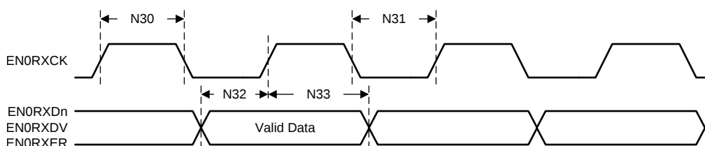
图 5-38. 100-Mbps MII Receive Timing
