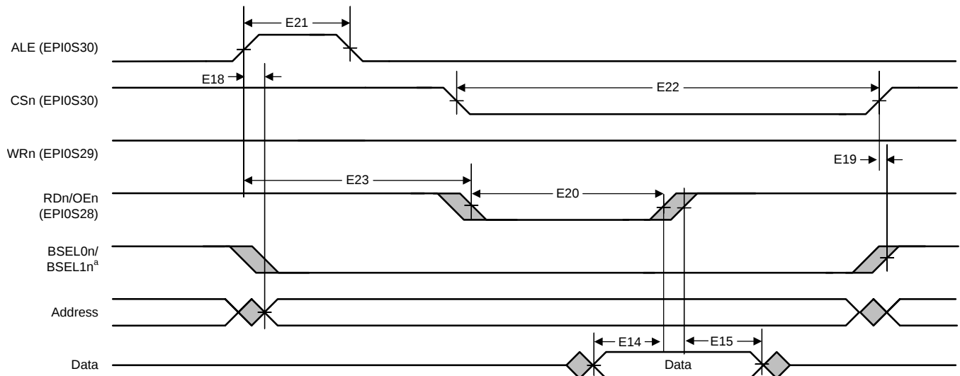
図 5-19. Host-Bus 8/16 Asynchronous Mode Read Timing
