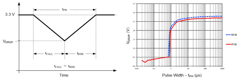
5-5. POR-BOR V_{DD} Glitch Response
