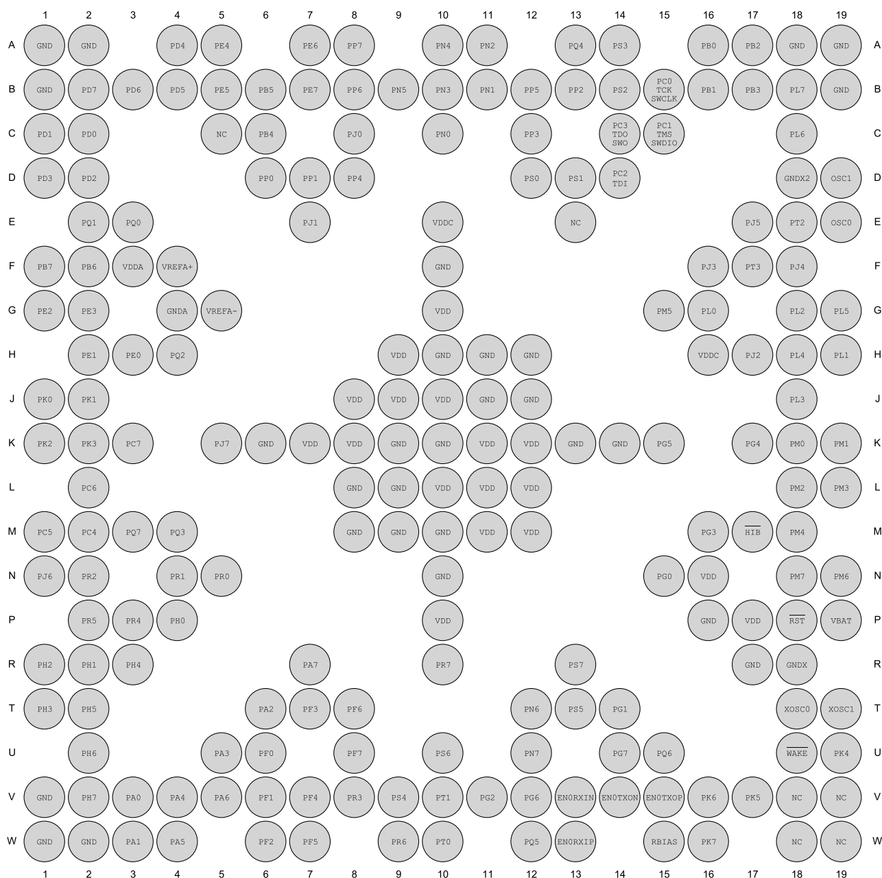
Figure 4-1. 212-Pin ZAD Package (Top View)
