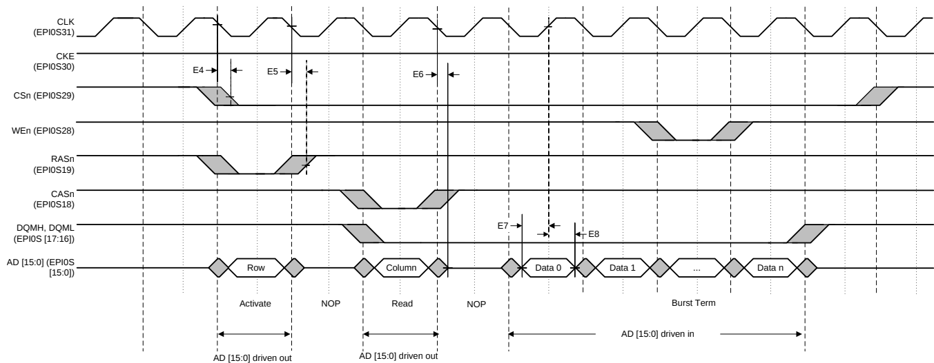
FIG 5-17. SDRAM Read Timing
