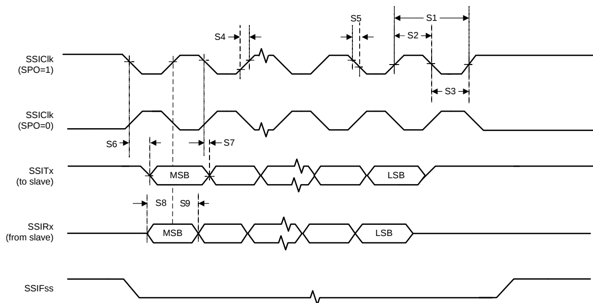
✎ 5-29. Master Mode SSI Timing for SPI Frame Format (FRF = 00), With SPH = 1
