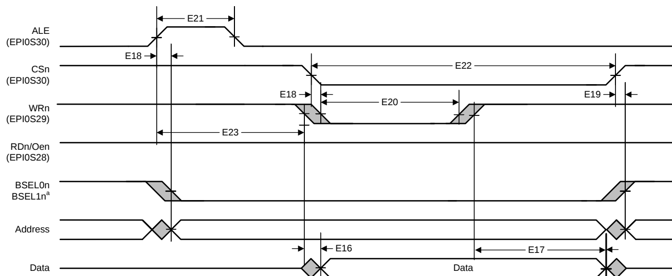
5-20. Host-Bus 8/16 Asynchronous Mode Write Timing
