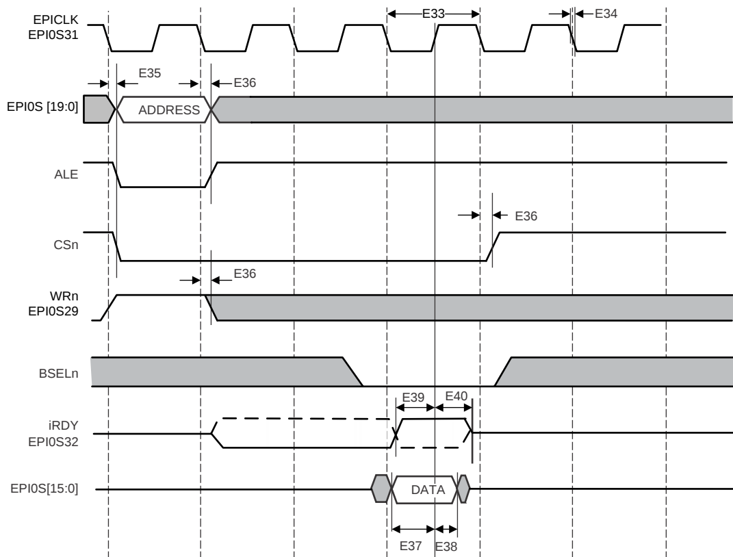
図 5-24. PSRAM Single Burst Read
