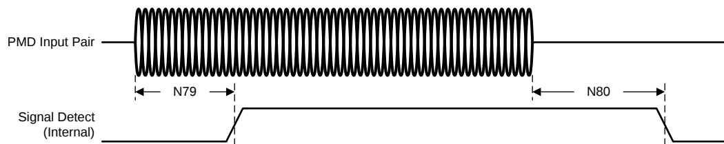
図 5-38. 100Base-TX Signal Detect Timing
