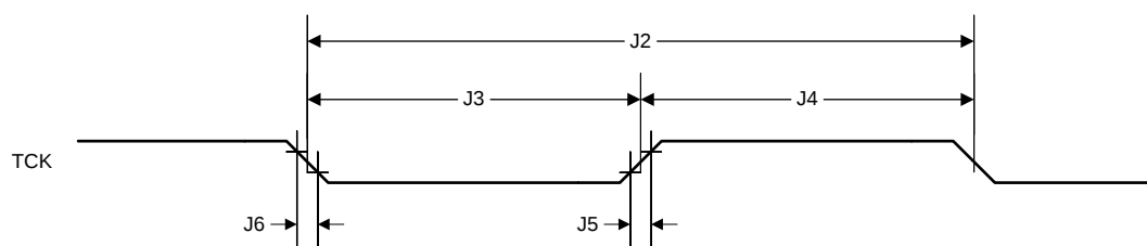
图 5-40. JTAG Test Clock Input Timing
