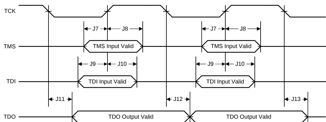
图 5-41. JTAG Test Access Port (TAP) Timing
