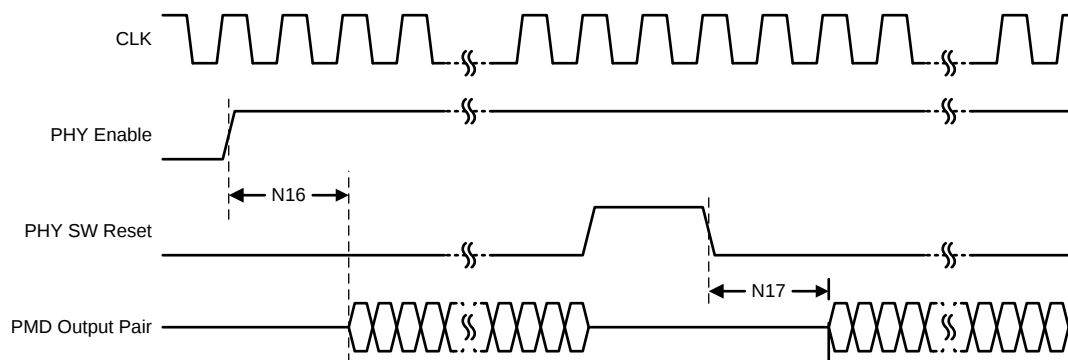
図 5-34. Reset Timing
