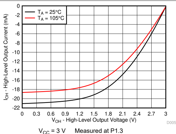
8-7. Typical High-Level Output Current vs High-Level Output Voltage
