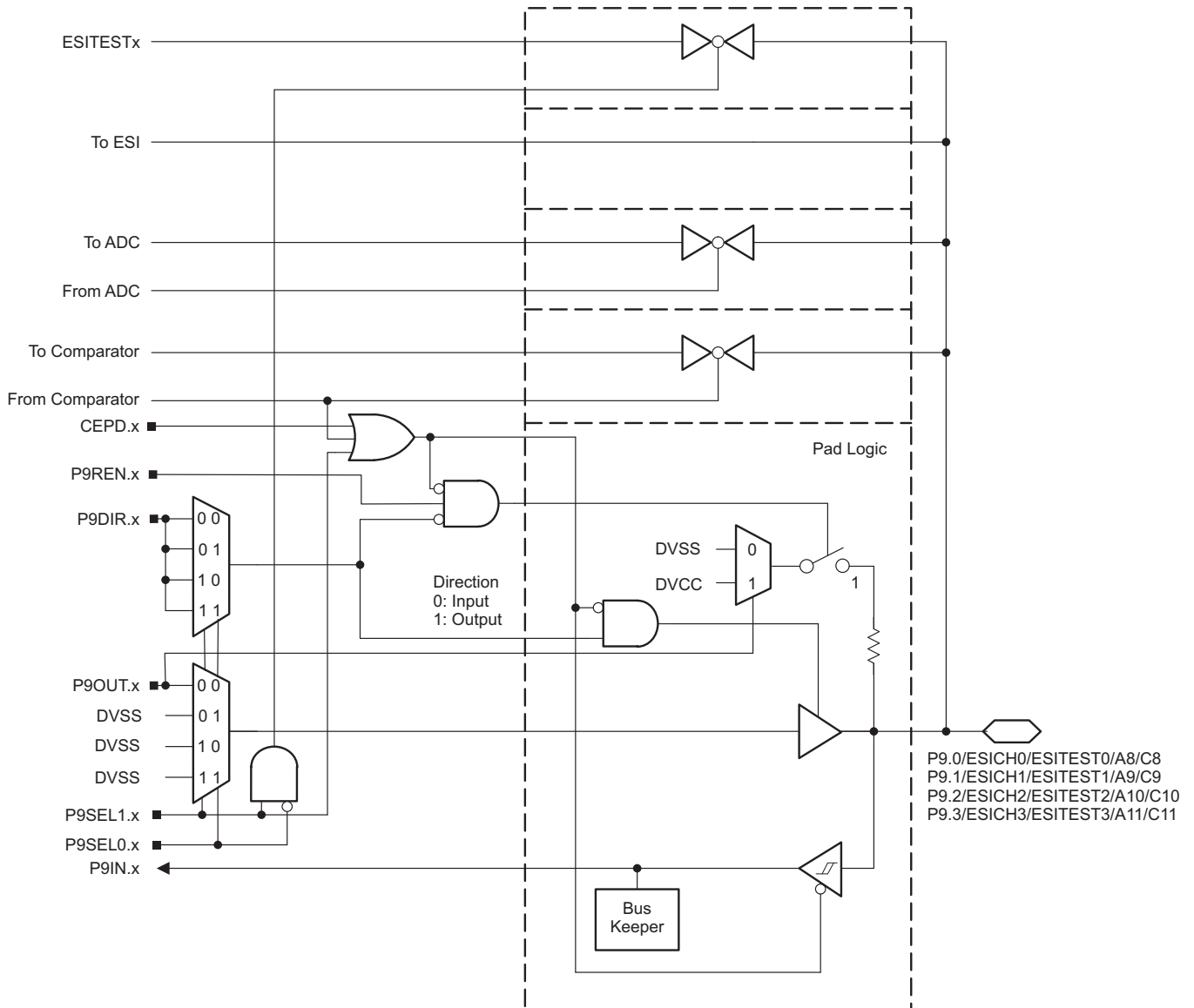
✎ 6-8. Port P9 (P9.0 to P9.3) Diagram
