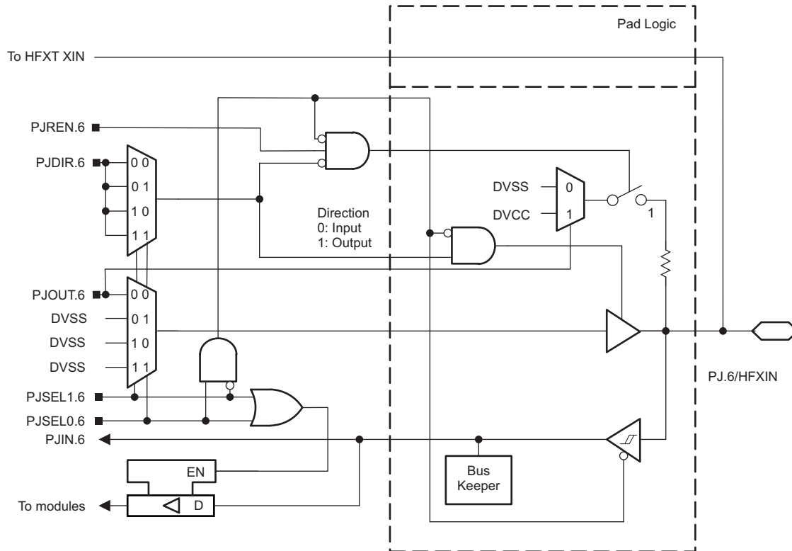
☒ 6-12. Port PJ (PJ.6) Diagram
