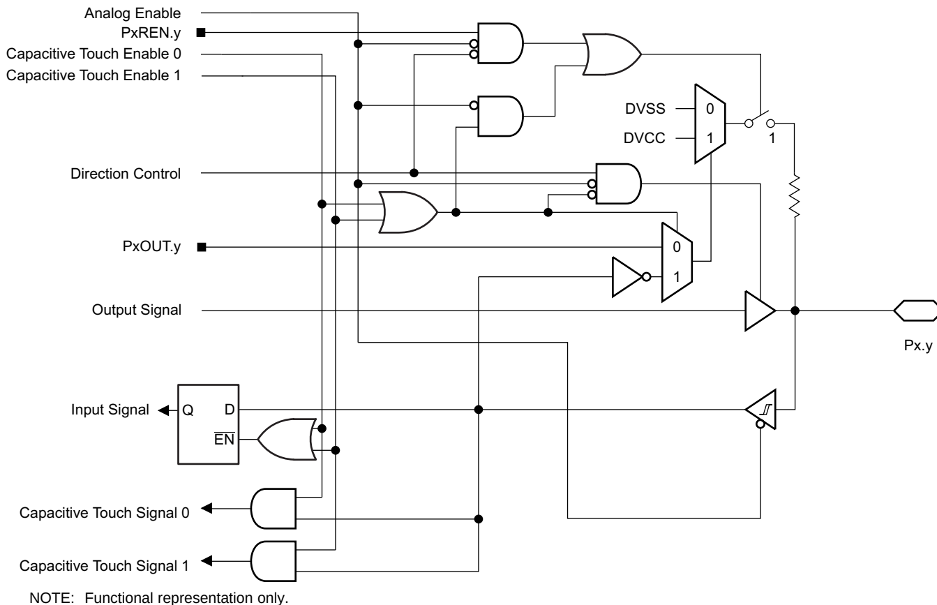
☒ 6-3. Capacitive Touch I/O Diagram
