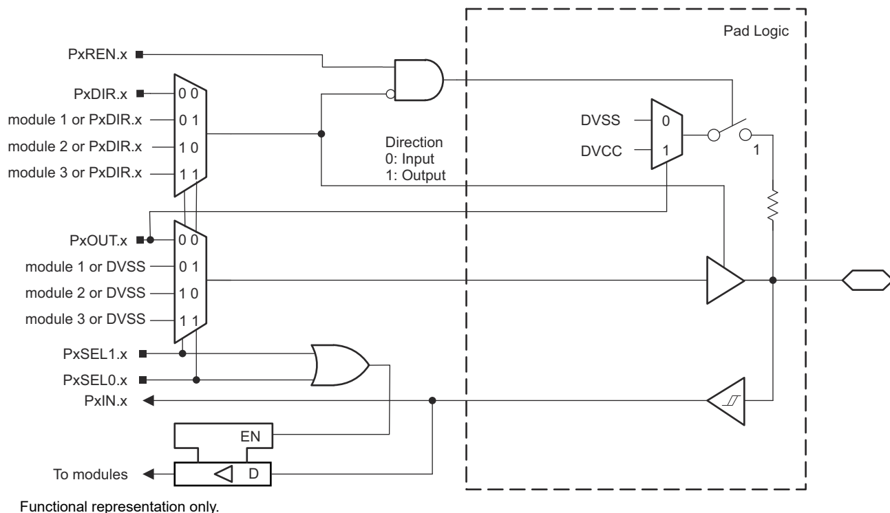
Figure 9-15. Port P8 (P8.0 to P8.3) Diagram
