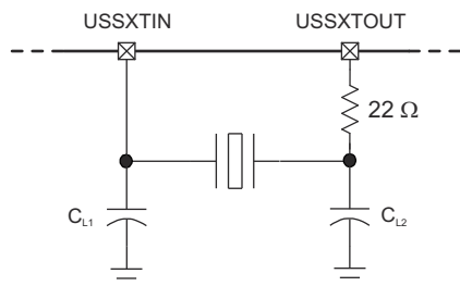
図 10-4. Typical Crystal Connection
