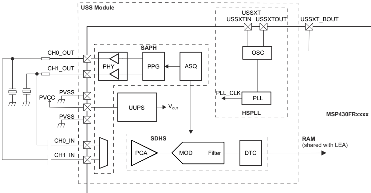
FIG 9-1. USS Subsystem Block Diagram
