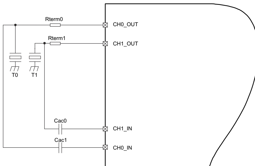
FIG 10-6. Typical Transducer Connection
