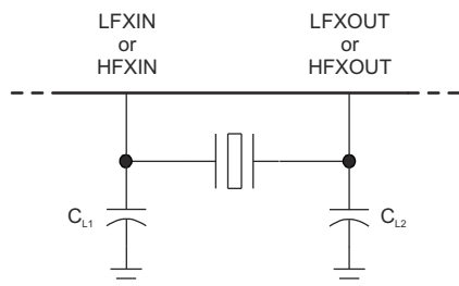
図 10-3. Typical Crystal Connection
