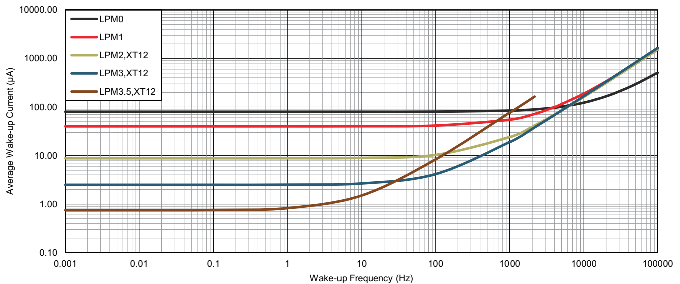
8-7. Average LPM Currents vs Wake-up Frequency at 85°C
