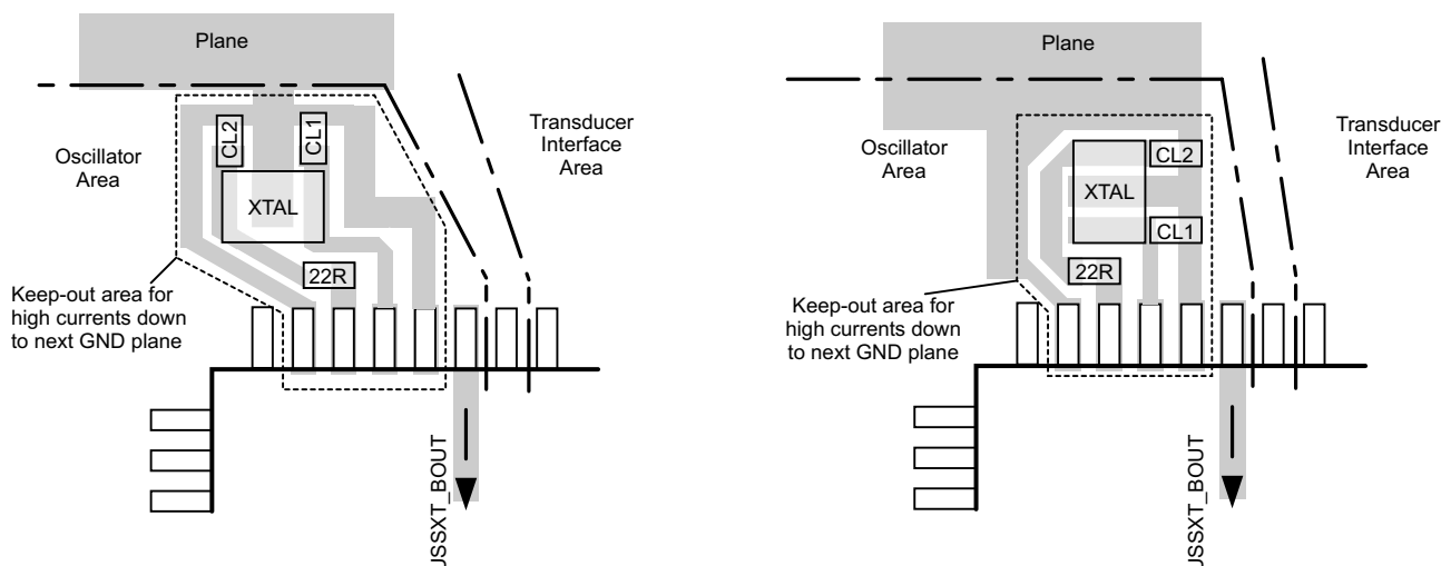
FIG 10-5. USSXT PCB Layout Recommendation
