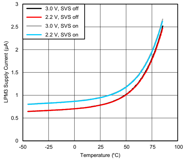
8-2. LPM3 Supply Current ( I_{LPM3,XT3.7} ) vs Temperature
