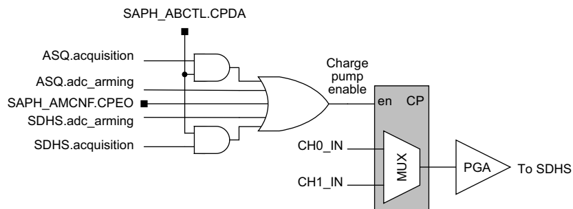
FIG 10-7. Control Of Input Multiplexer
