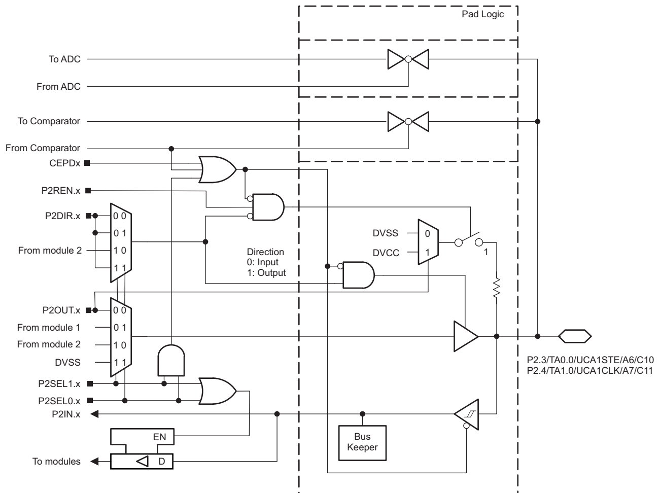
❏ 5-6. Port P2 (P2.3 and P2.4) Diagram
