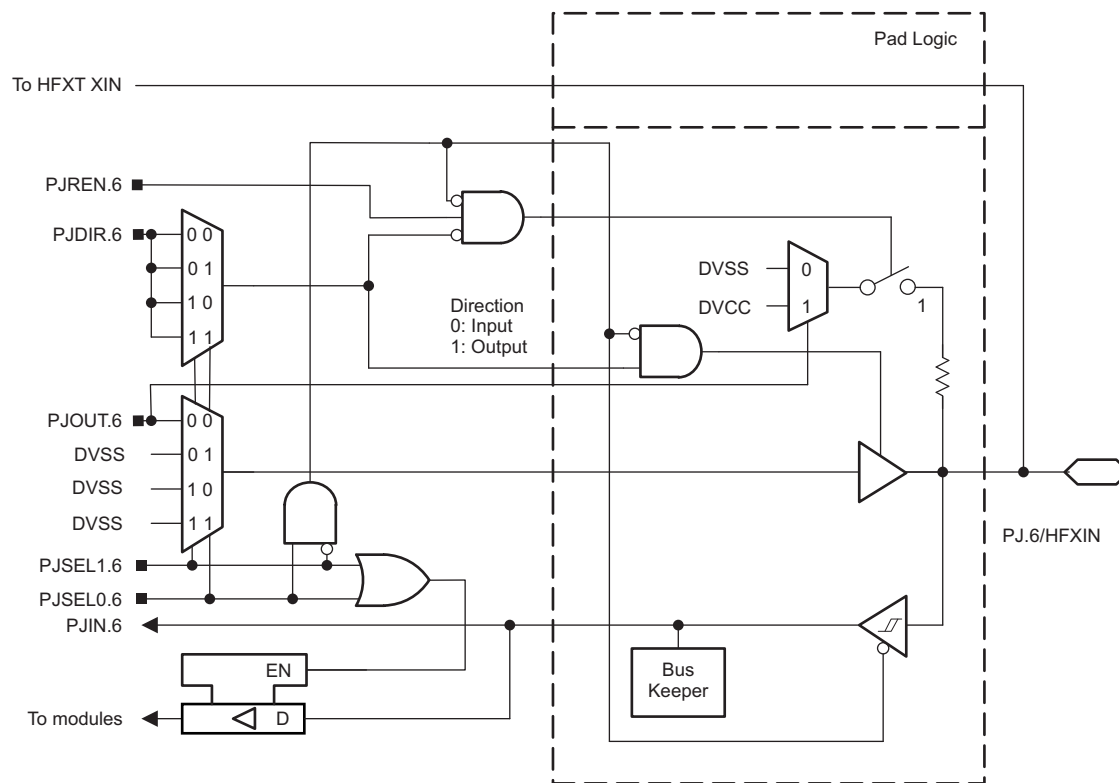
☒ 6-16. Port PJ (PJ.6) Diagram
