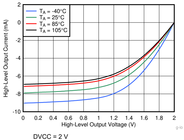
8-10. Typical High-Level Output Current vs High-Level Output Voltage
