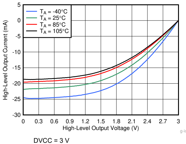
8-9. Typical High-Level Output Current vs High-Level Output Voltage
