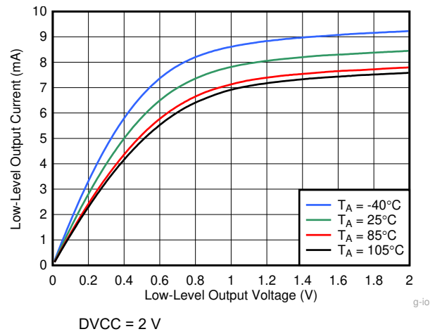
8-8. Typical Low-Level Output Current vs Low-Level Output Voltage
