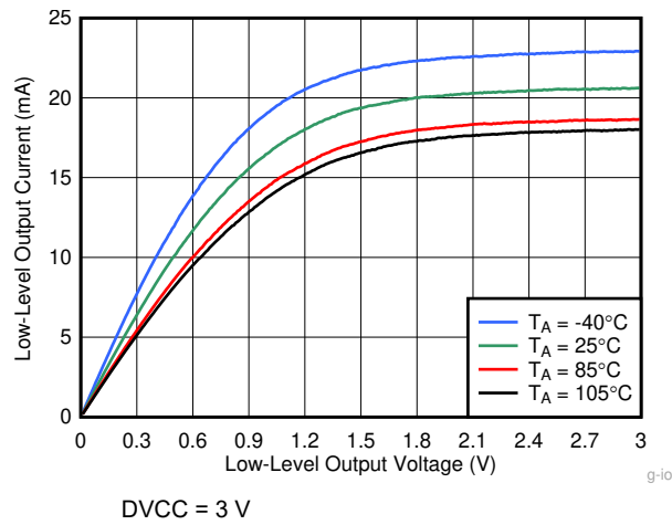
8-7. Typical Low-Level Output Current vs Low-Level Output Voltage
