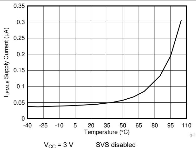
FIG 8-4. LPM4.5 Supply Current vs Temperature
