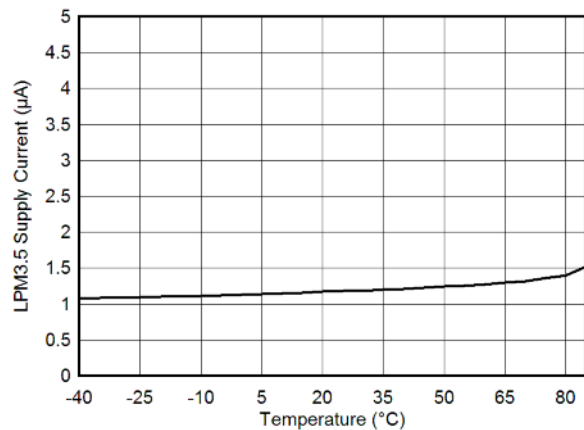
FIG 8-3. LPM3.5 Supply Current vs Temperature
