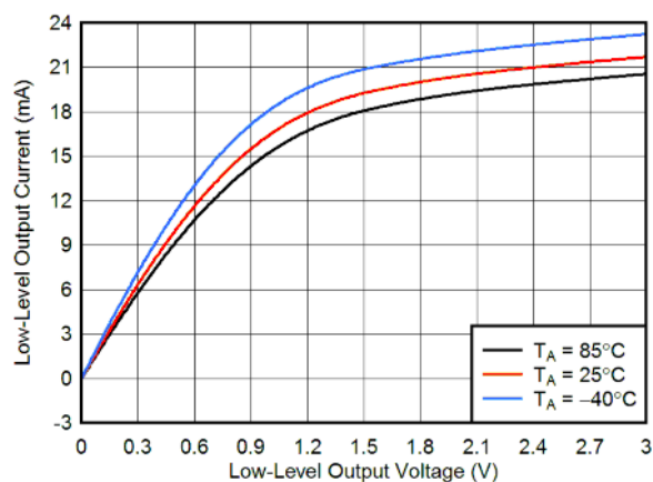
FIG 8-7. Typical Low-Level Output Current vs Low-Level Output Voltage
