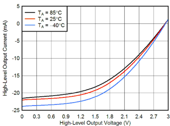
FIG 8-9. Typical High-Level Output Current vs High-Level Output Voltage
