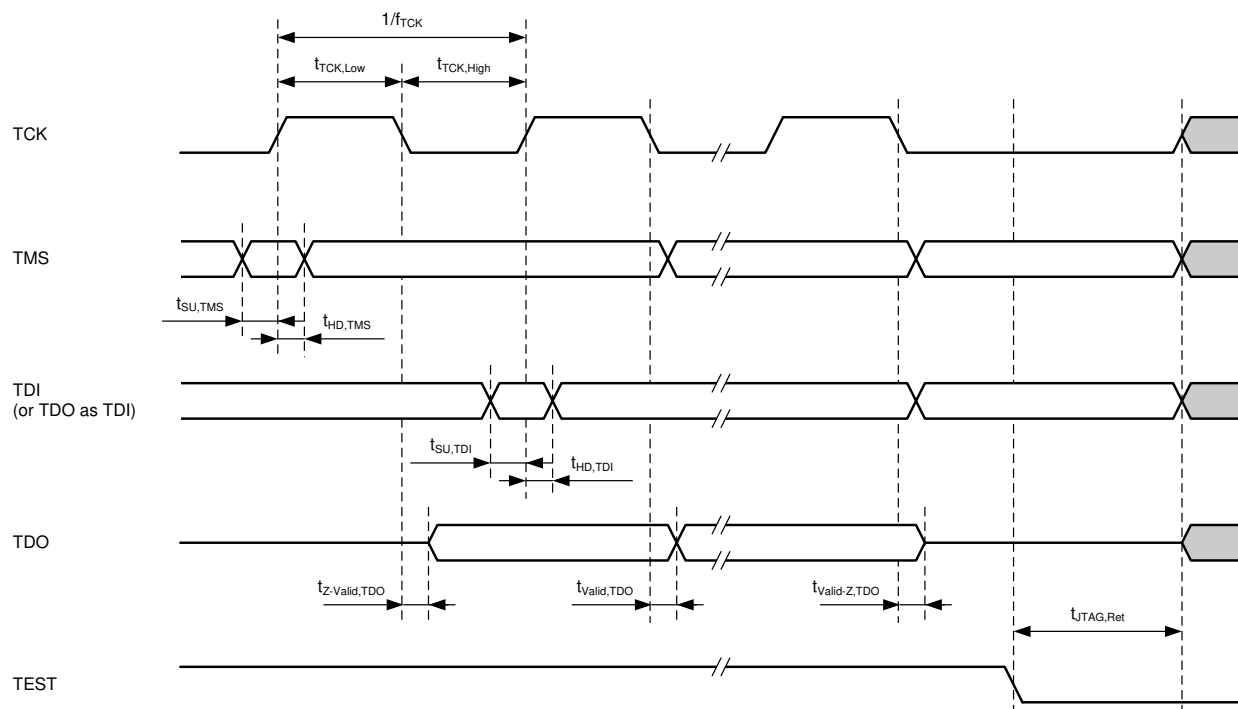
図 8-19. JTAG 4-Wire Timing
