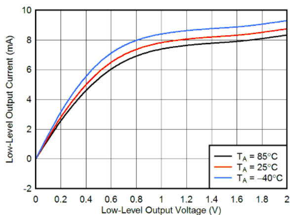
FIG 8-8. Typical Low-Level Output Current vs Low-Level Output Voltage
