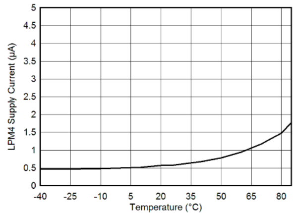
FIG 8-2. LPM4 Supply Current vs Temperature
