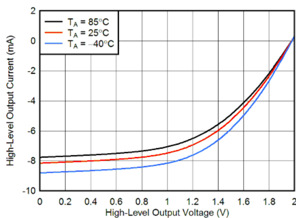
FIG 8-10. Typical High-Level Output Current vs High-Level Output Voltage
