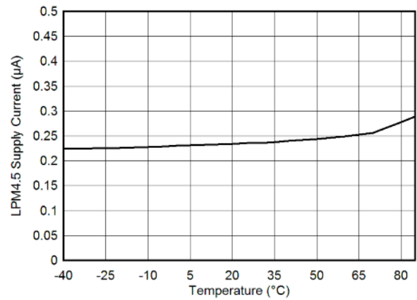
FIG 8-4. LPM4.5 Supply Current vs Temperature
