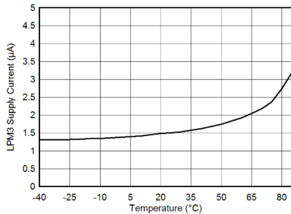
FIG 8-1. LPM3 Supply Current vs Temperature
