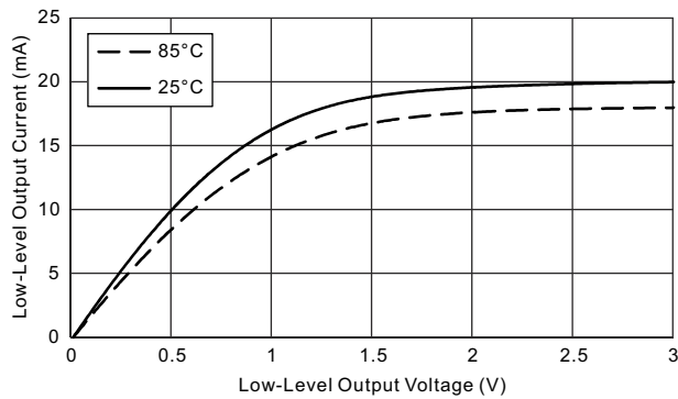
FIG 8-6. Typical Low-Level Output Current vs Low-Level Output Voltage (DVCC = 3 V)
