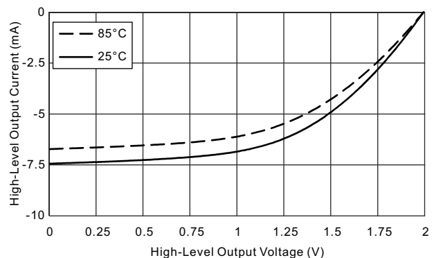
FIG 8-9. Typical High-Level Output Current vs High-Level Output Voltage (DVCC = 2 V)
