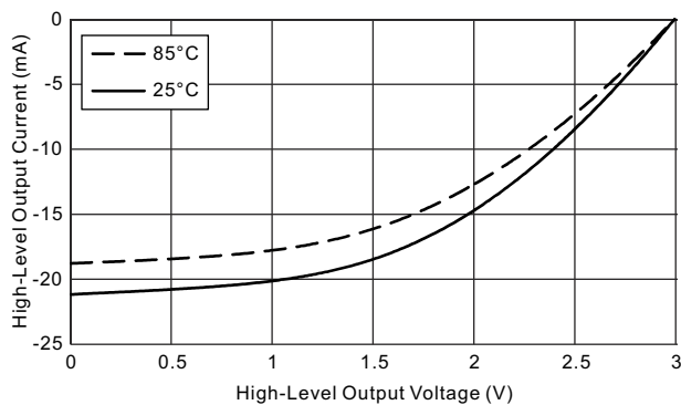
FIG 8-8. Typical High-Level Output Current vs High-Level Output Voltage (DVCC = 3 V)
