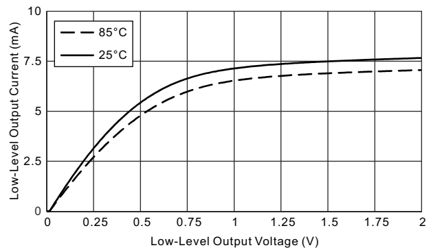
FIG 8-7. Typical Low-Level Output Current vs Low-Level Output Voltage (DVCC = 2 V)
