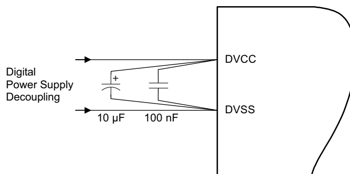
図 10-1. Power Supply Decoupling
