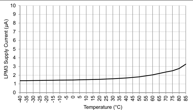
DVCC = 3 V RTC Enabled SVS Disabled FIG 8-1. Low-Power Mode 3 Supply Current vs Temperature
