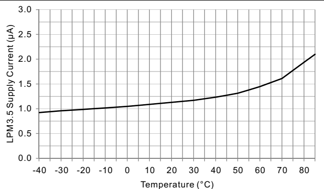
DVCC = 3 V XT1, 12.5-pF Crystal SVS Enabled FIG 8-2. LPM3.5 Supply Current vs Temperature
