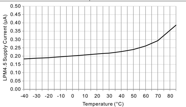
DVCC = 3 V SVS Enabled FIG 8-3. LPM4.5 Supply Current vs Temperature
