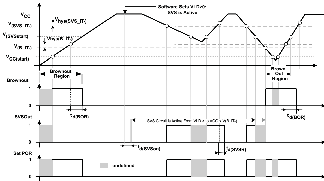
Figure 5-13. SVS Reset (SVSR) vs Supply Voltage
