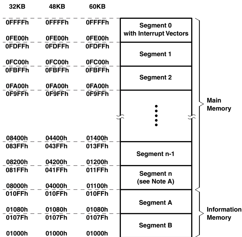
9-7. Flash Memory Segments
