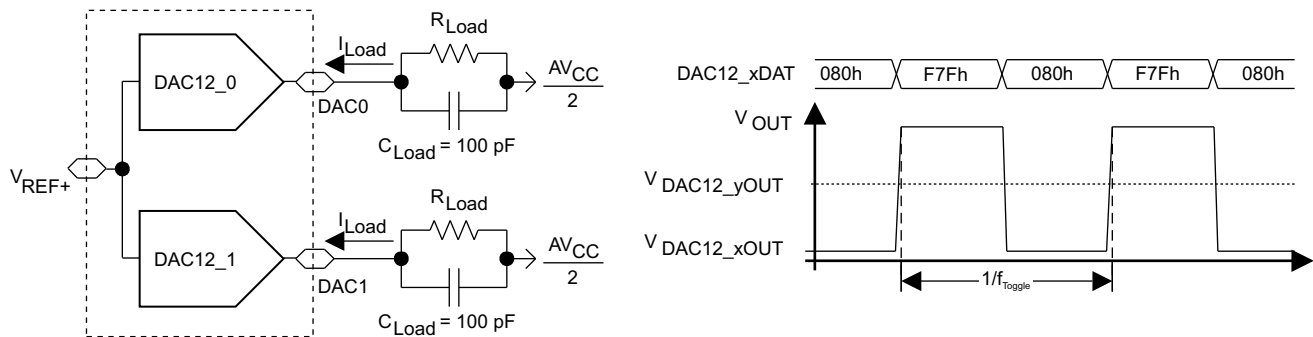
FIG 8-28. Crosstalk Test Conditions
