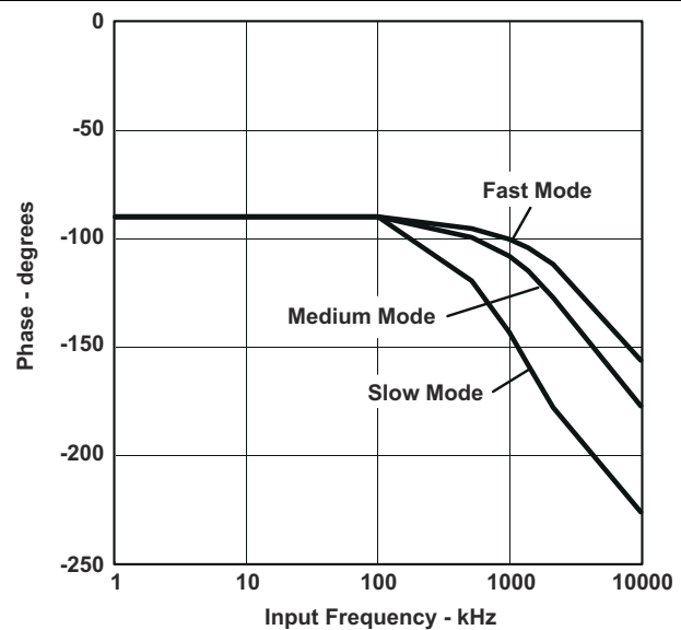
8-31. Typical Phase vs Frequency
