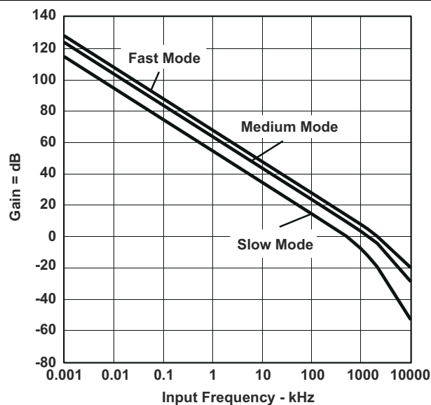
8-30. Typical Open-Loop Gain vs Frequency
