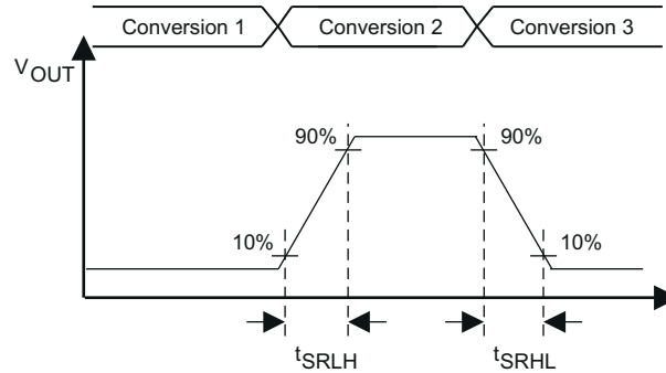
FIG 8-26. Slew Rate Testing
