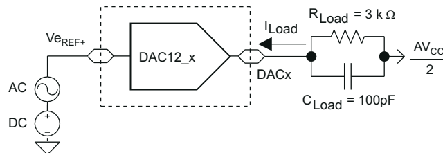
FIG 8-27. Test Conditions for 3-dB Bandwidth Specification
