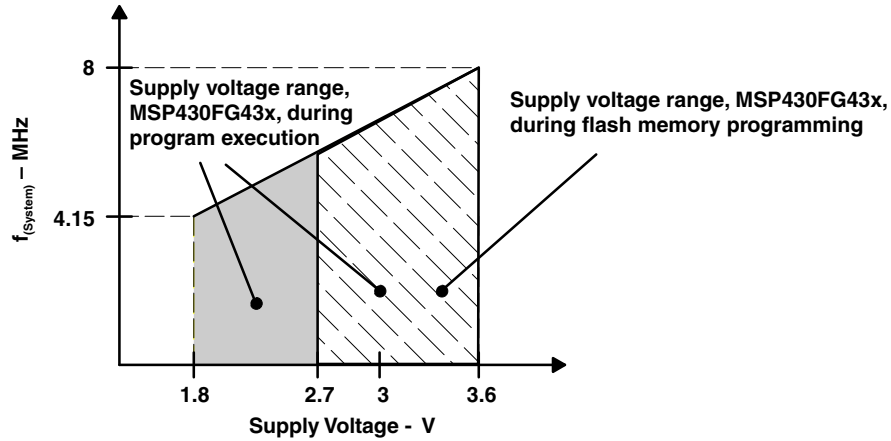
8-1. Frequency vs Supply Voltage, Typical Characteristic
