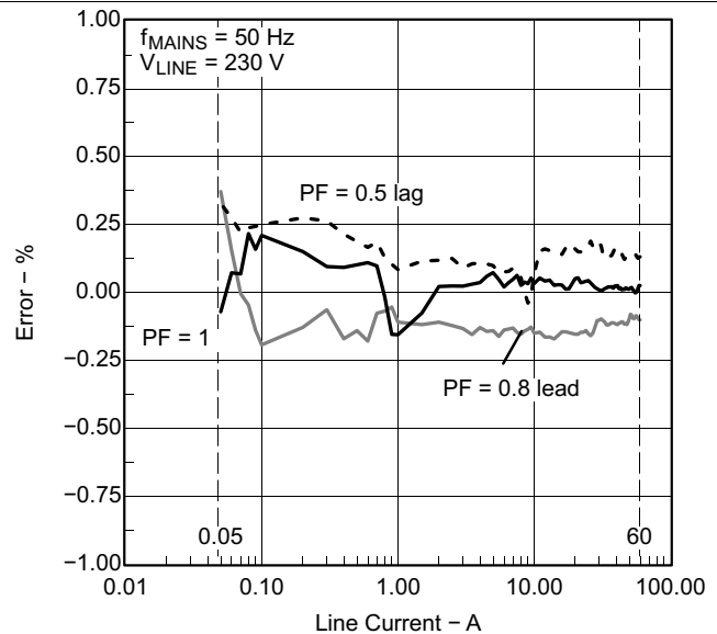
Figure 5-26. Measurement Error as Percentage of Reading ( T_A = -40^\circ\text{C} )
