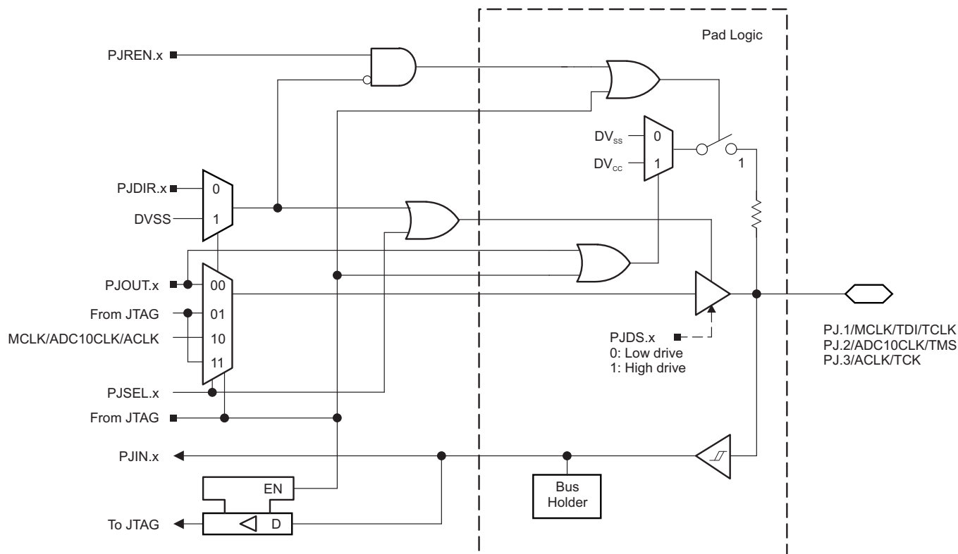
☒ 6-18. Port PJ (PJ.1 to PJ.3) Diagram
