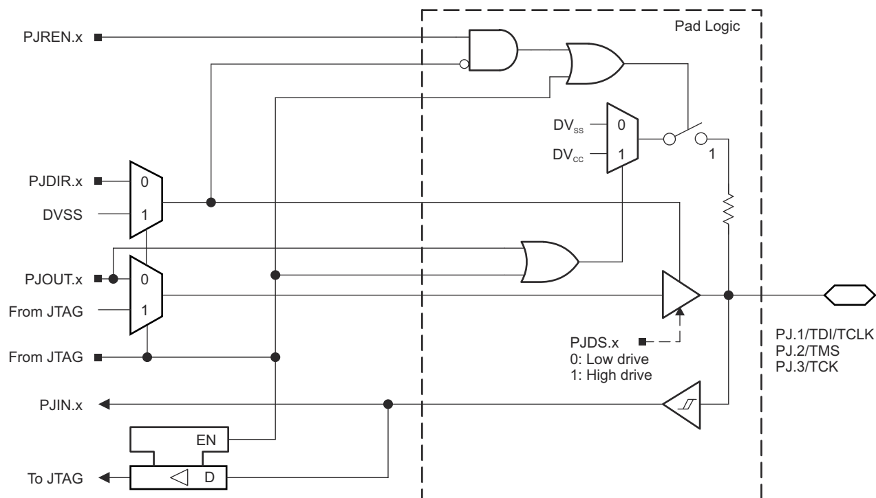
9-16. Port PJ (PJ.1 to PJ.3) Diagram
