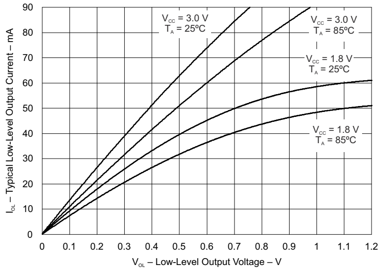
8-23. Ports PU.0, PU.1 Typical Low-Level Output Characteristics
