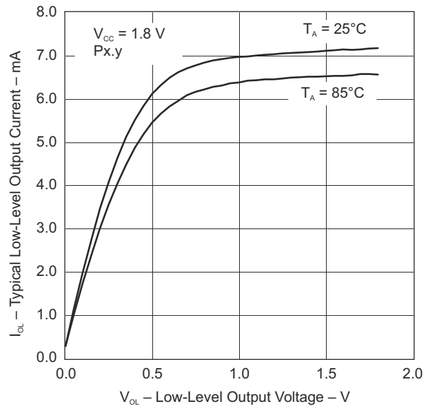
7-4. Typical Low-Level Output Current vs Low-Level Output Voltage
