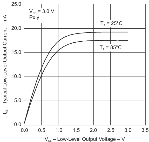
7-3. Typical Low-Level Output Current vs Low-Level Output Voltage
