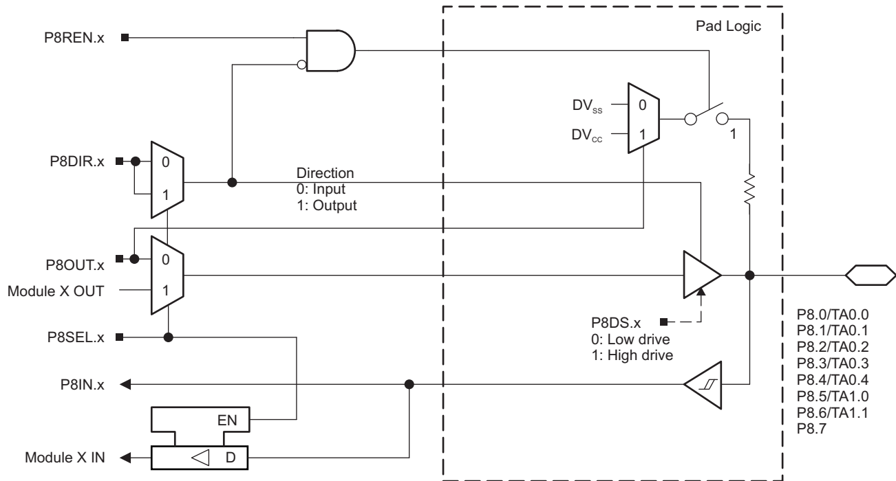
Figure 6-15. Port P8 (P8.0 to P8.7) Diagram
