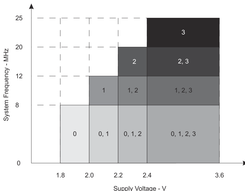
8-1. Frequency vs Supply Voltage
