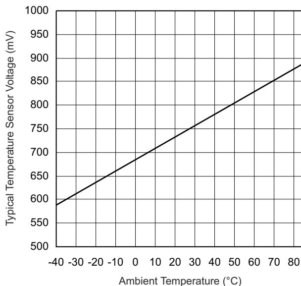
FIG 8-16. Typical Temperature Sensor Voltage
