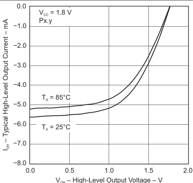
8-7. Typical High-Level Output Current vs High-Level Output Voltage
