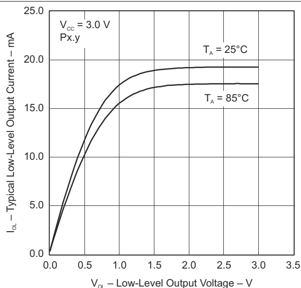
8-4. Typical Low-Level Output Current vs Low-Level Output Voltage
