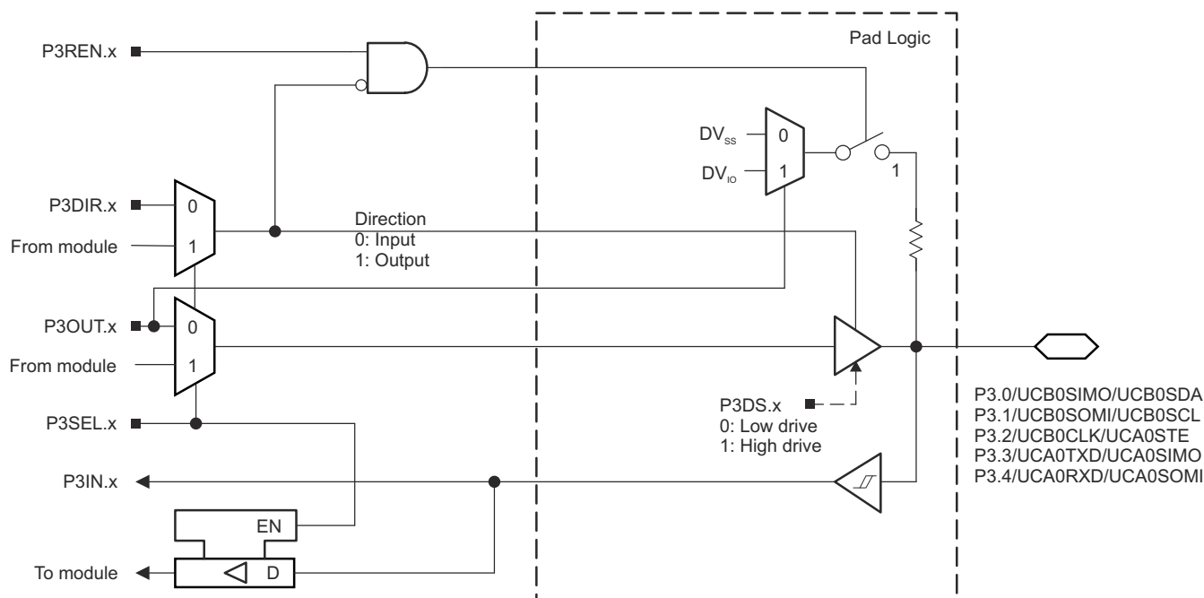
9-4. Port P3 (P3.0 to P3.4) Diagram
