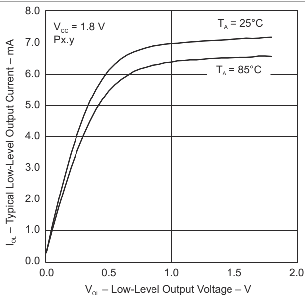
8-5. Typical Low-Level Output Current vs Low-Level Output Voltage
