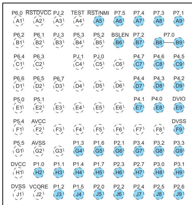
7-2. 80-Pin ZXH or ZQE Package (Top View)
