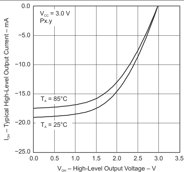
8-6. Typical High-Level Output Current vs High-Level Output Voltage
