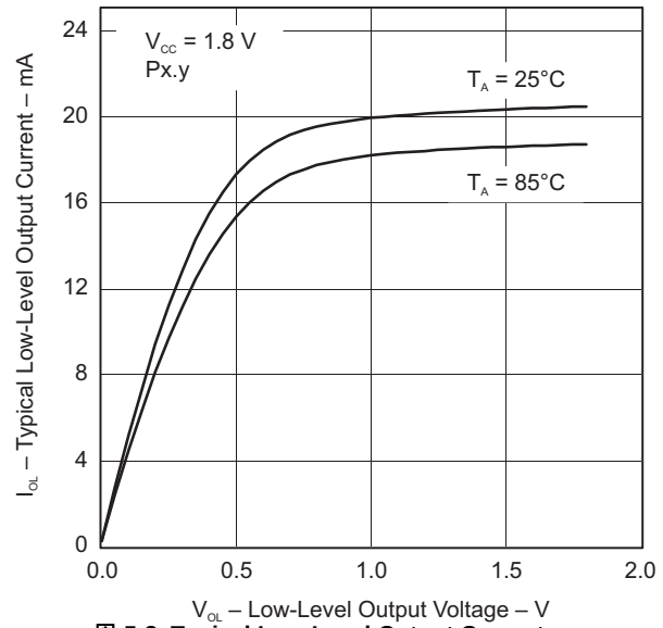
FIG 5-8. Typical Low-Level Output Current vs Low-Level Output Voltage
