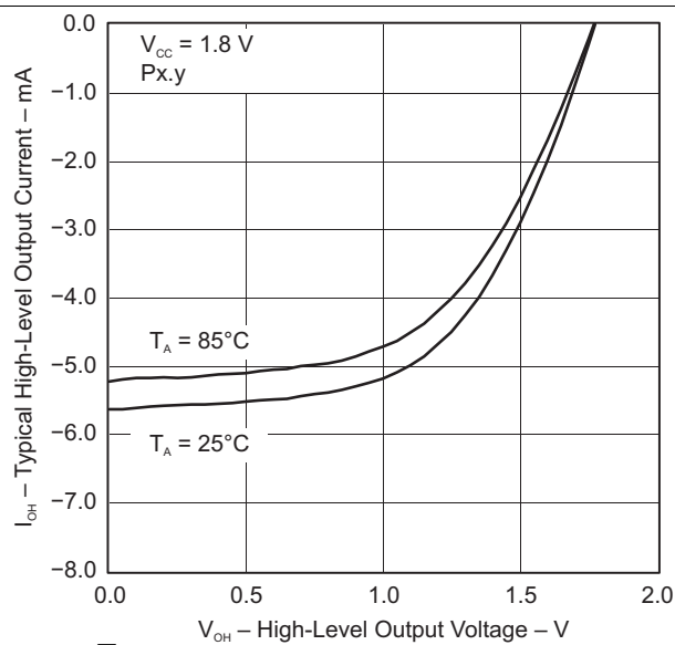
FIG 5-6. Typical High-Level Output Current vs High-Level Output Voltage
