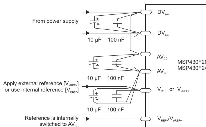
8-40. Supply Voltage and Reference Voltage Design V_{REF}/V_{REF-} = AV_{SS} , Internally Connected
