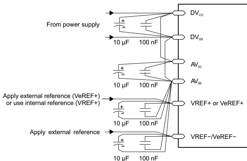
Figure 5-14. Supply Voltage and Reference Voltage Design, V_{REF-}/V_{eREF-} External Supply
