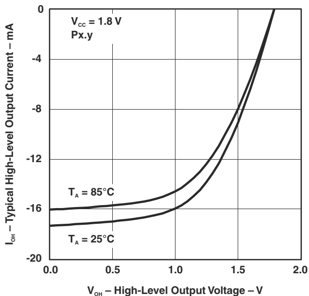
Figure 7-5. Typical High-Level Output Current vs High-Level Output Voltage
