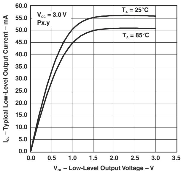
Figure 7-2. Typical Low-Level Output Current vs Low-Level Output Voltage
