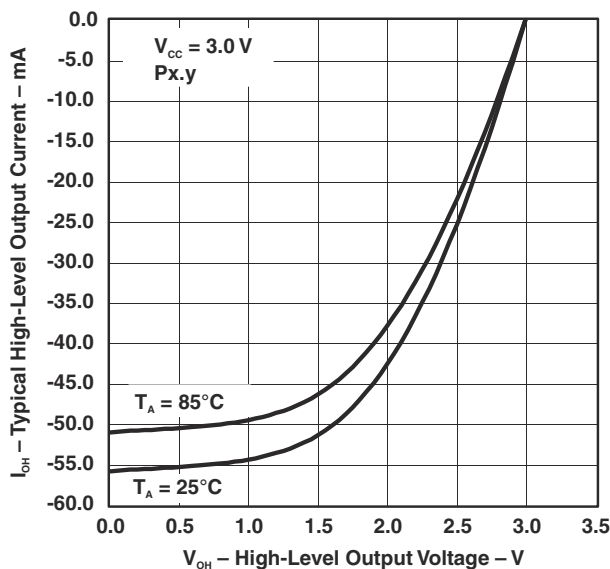
Figure 7-4. Typical High-Level Output Current vs High-Level Output Voltage
