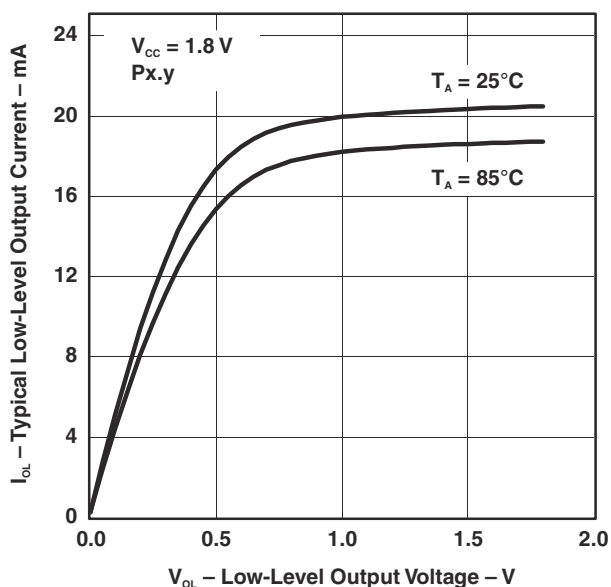
Figure 7-3. Typical Low-Level Output Current vs Low-Level Output Voltage
