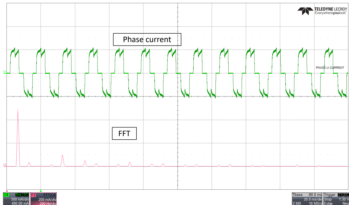
9-3. Phase current and FFT - 120 °commutation
