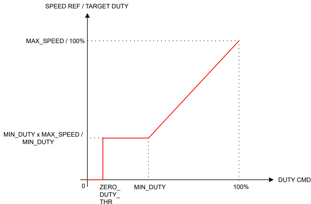
FIG 8-15. Speed Input Transfer Function
