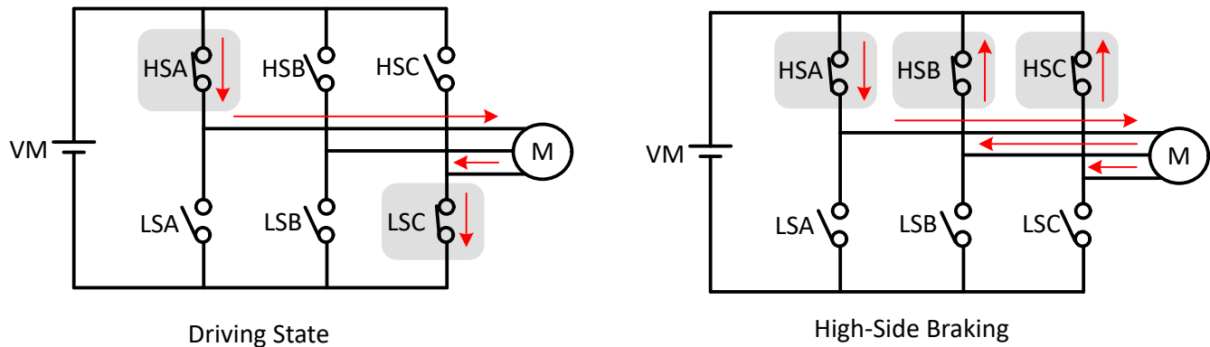
✎ 8-44. High-Side Braking
