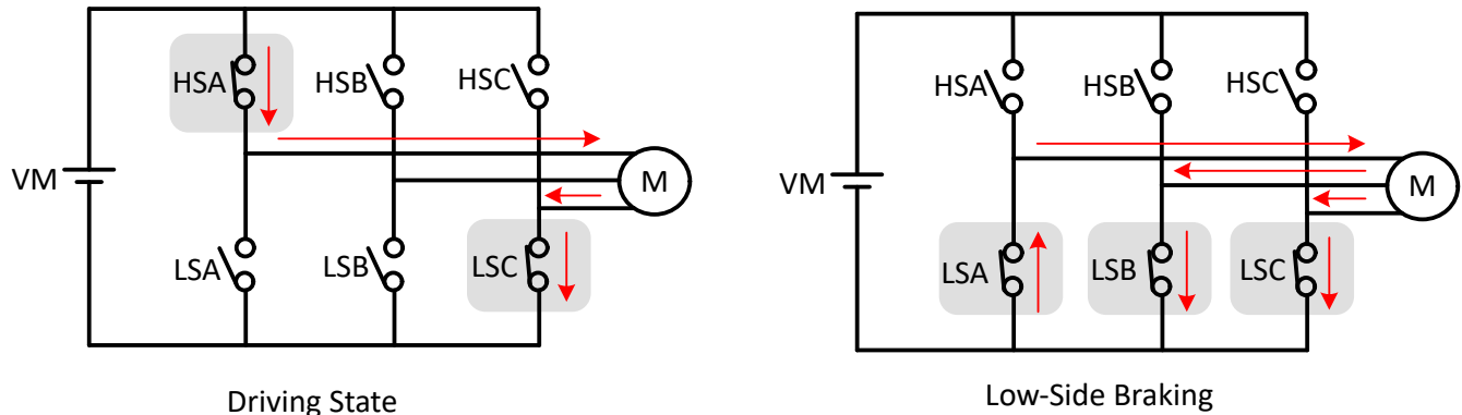
8-43. Low-Side Braking
