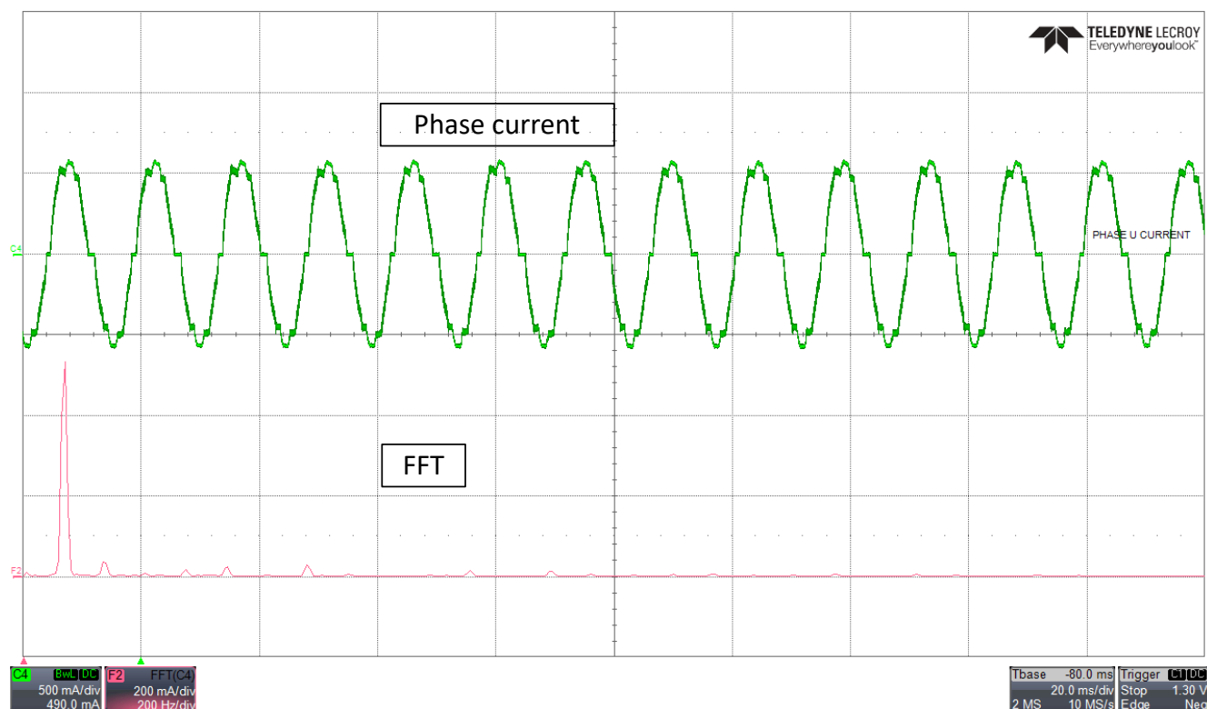
9-4. Phase current and FFT - 150°commutation
