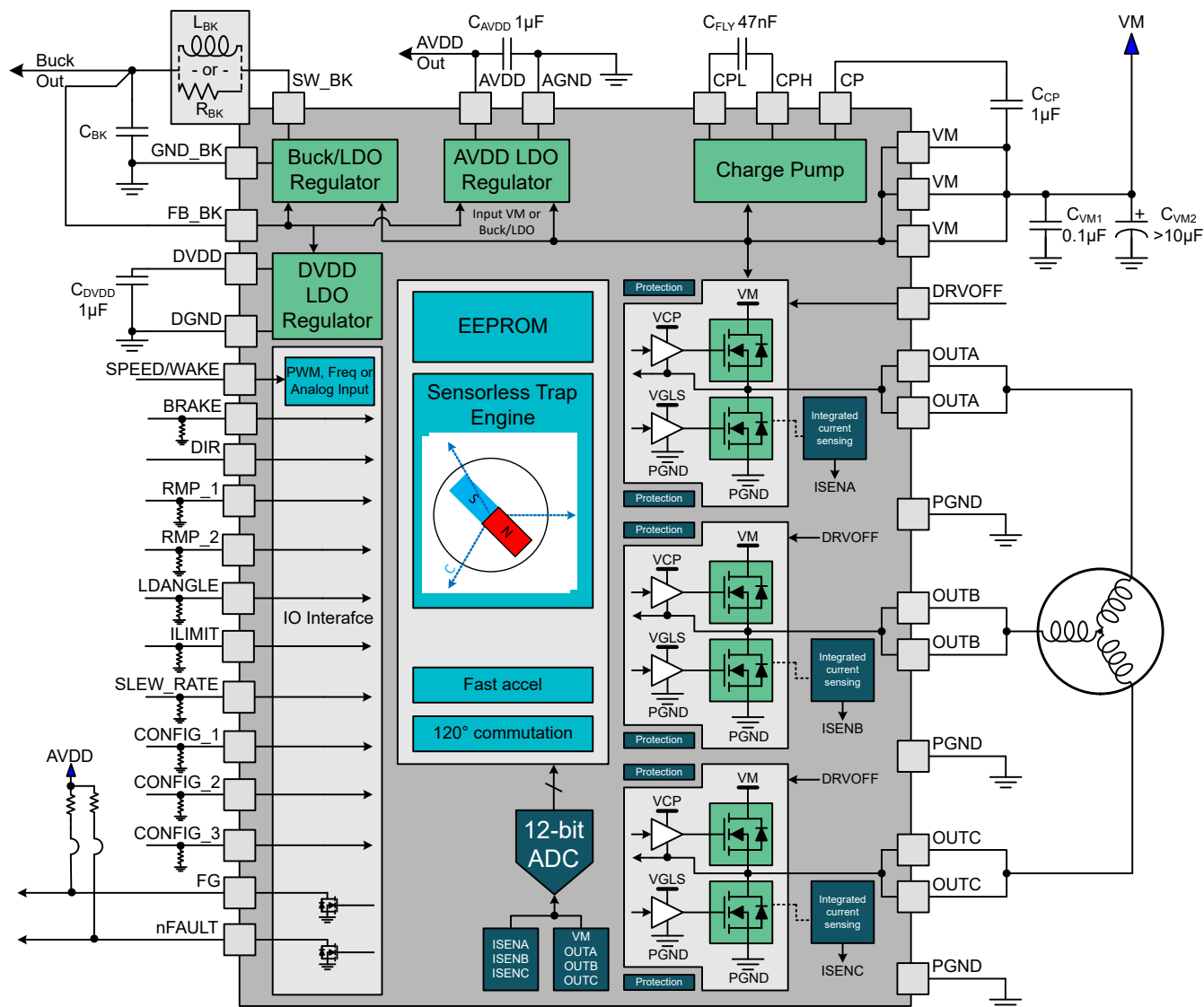
图 8-2. MCT8316AT Functional Block Diagram
