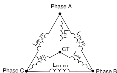
图 7-35. Motor Inductance
