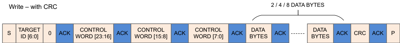
7-53. I 2 C Write Operation Sequence
