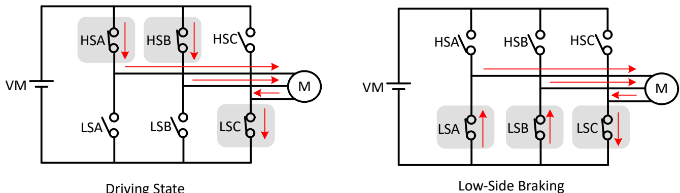
图 7-43. Low-Side Braking
