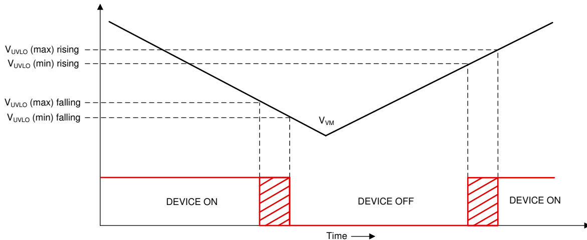
7-48. VM Supply Undervoltage Lockout
