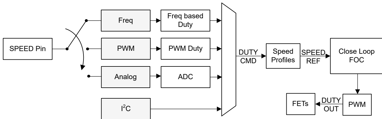
图 7-13. Multiplexing the Speed Command
