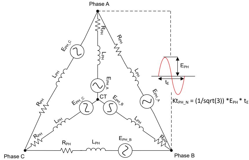
図 7-36. Motor back-EMF constant
