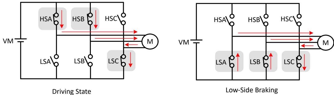
図 6-45. Low-Side Braking
