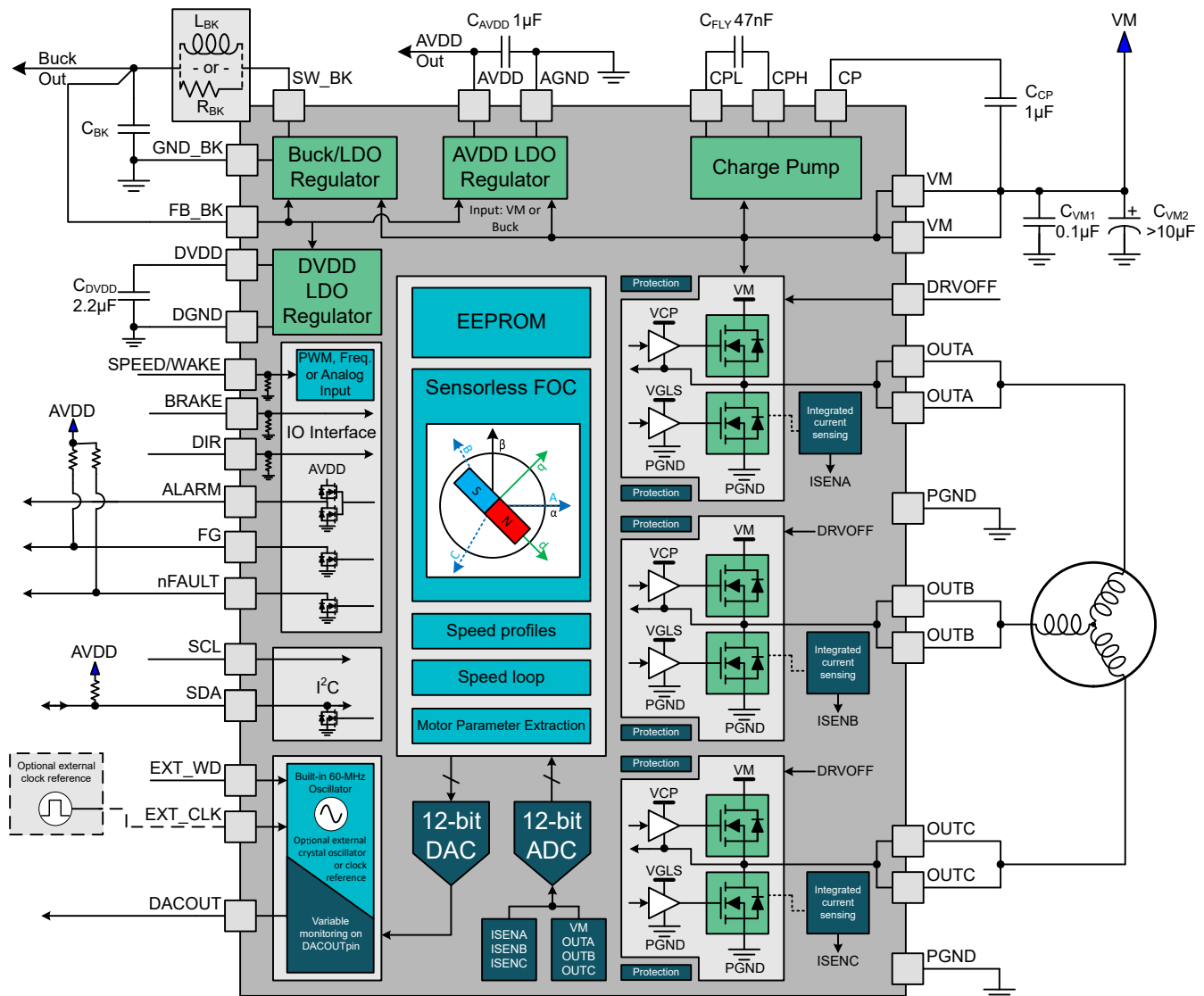
図 6-1. MCF8315C (RRY) Functional Block Diagram
