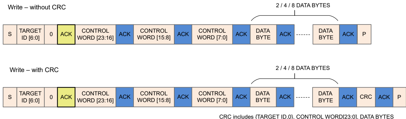
図 6-55. I 2 C Write Transaction Sequence
