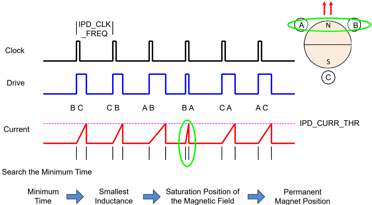
图 6-26. IPD Operation
