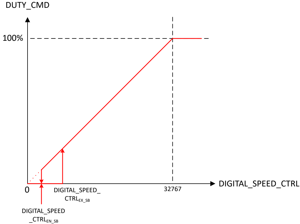
図 7-16. I2C Mode Speed Control
