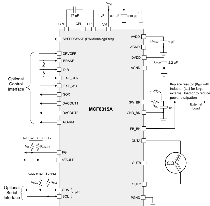
図 8-1. Example Application Schematic
