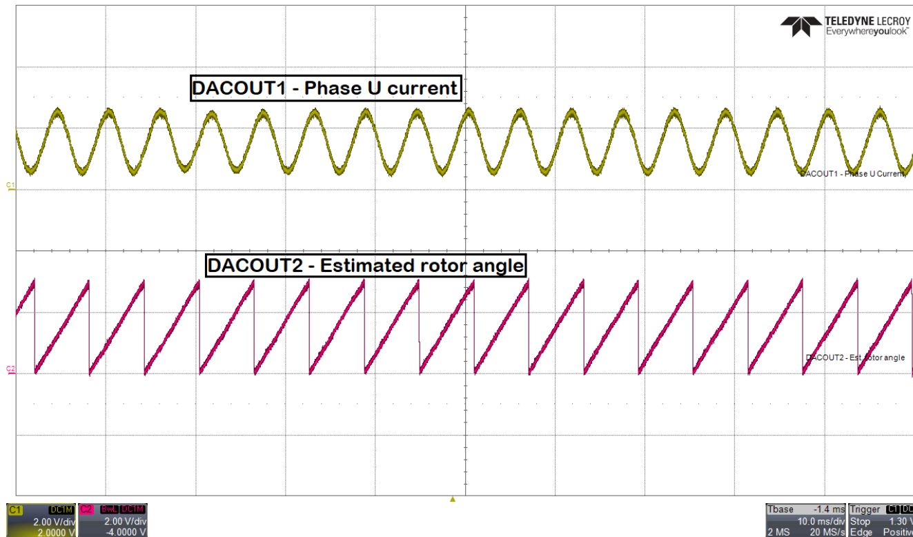
✎ 8-12. DACOUT1 and DACOUT2
