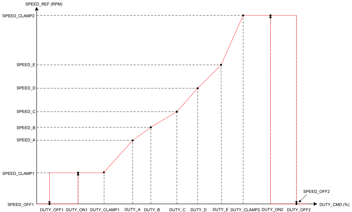
図 7-19. Linear Speed Profile
