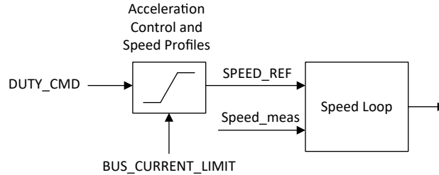
図 7-51. DC Bus Current Limit Functional Block Diagram
