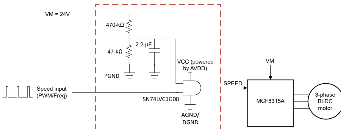
图 8-2. Delay circuit when speed command applied before VM power-up
