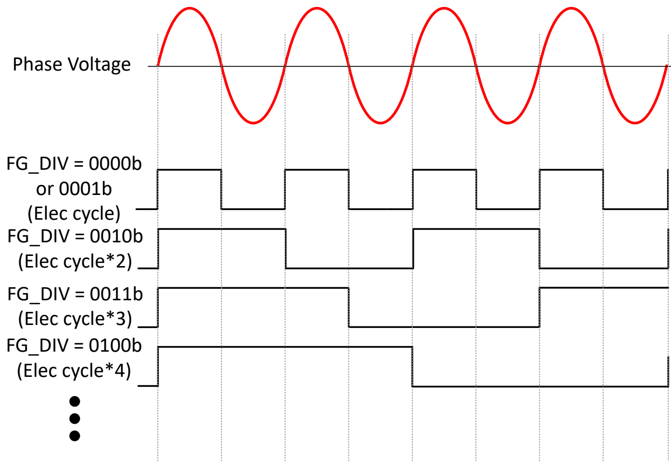
7-49. FG Frequency Divider
