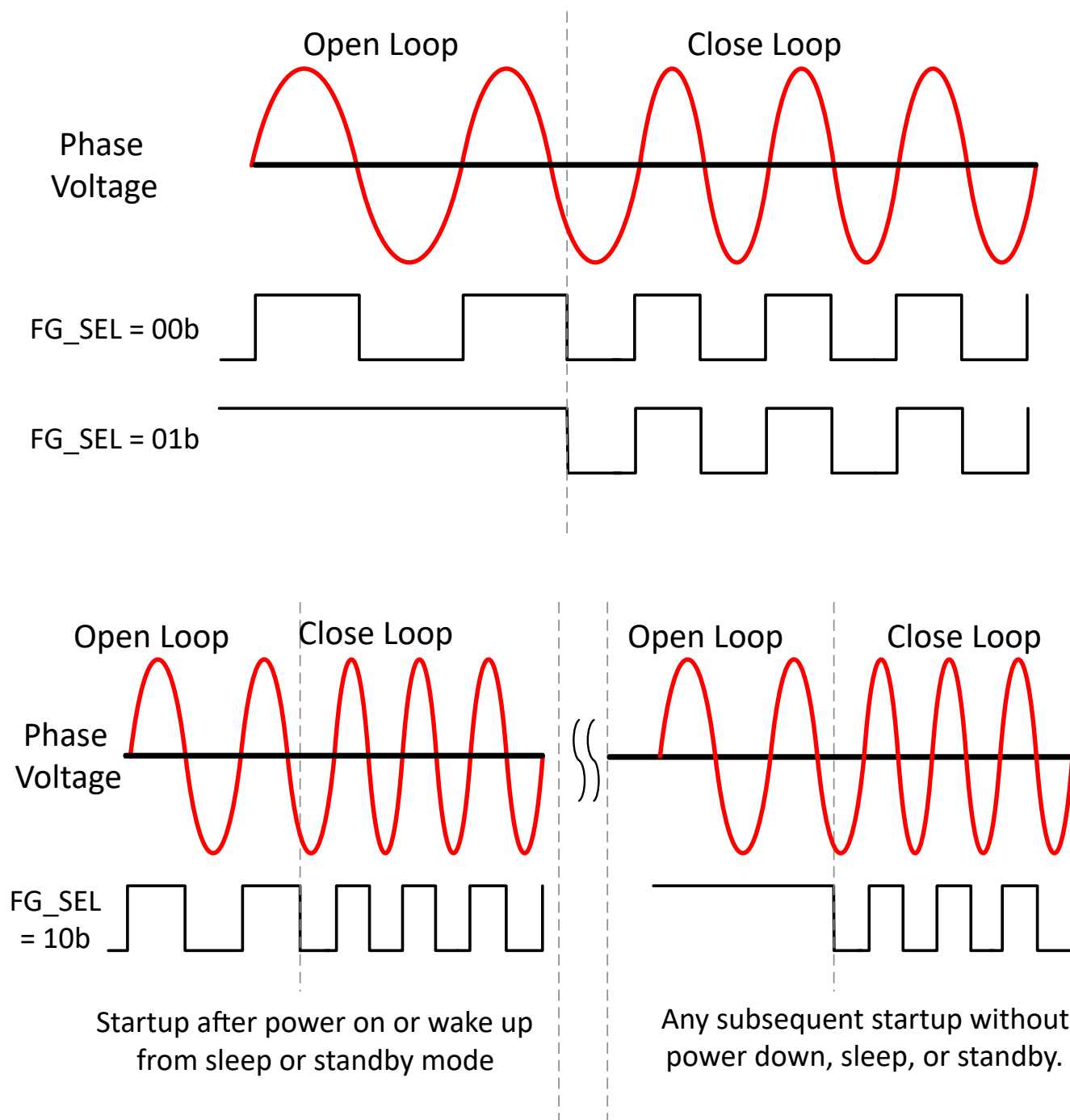
FIG 7-50. FG Behavior During Open Loop
