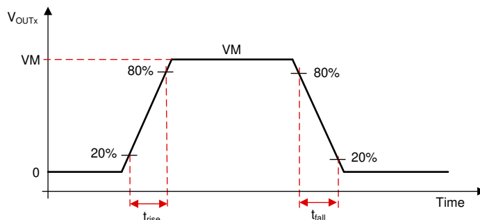
FIG 7-10. Slew Rate Timings
