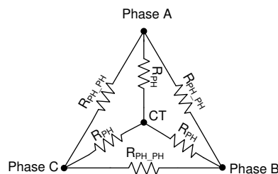
图 7-38. Motor Resistance
