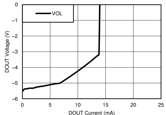
6-2. DOUT V_{OL} vs Load Current
