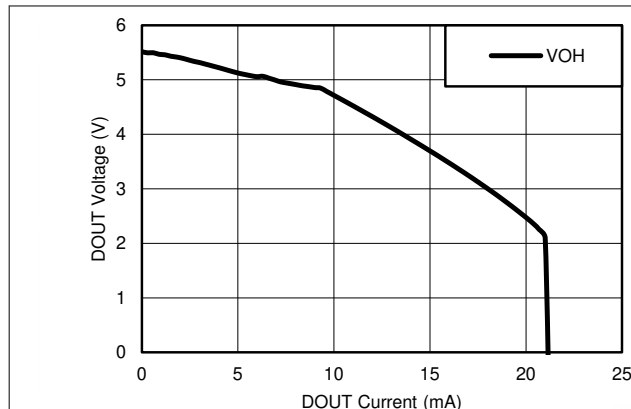
6-1. DOUT V_{OH} vs Load Current
