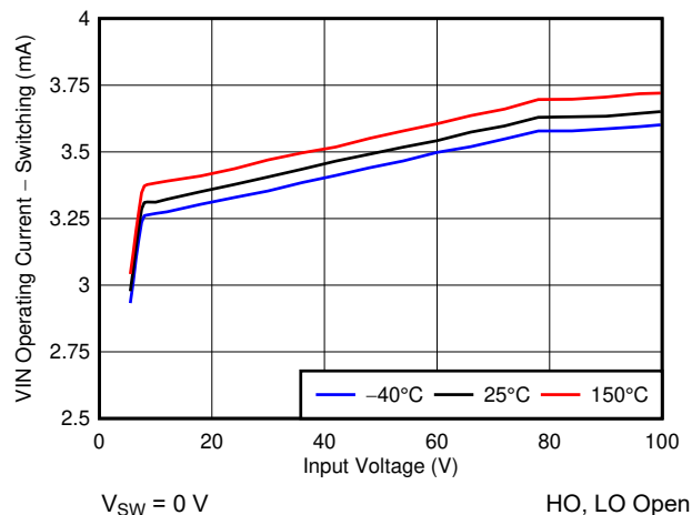
FIG 7-8. I_{Q-OPERATING} (Switching) vs Input Voltage
