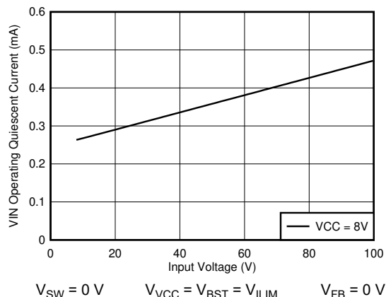
FIG 7-9. VIN Quiescent Current with External VCC Applied
