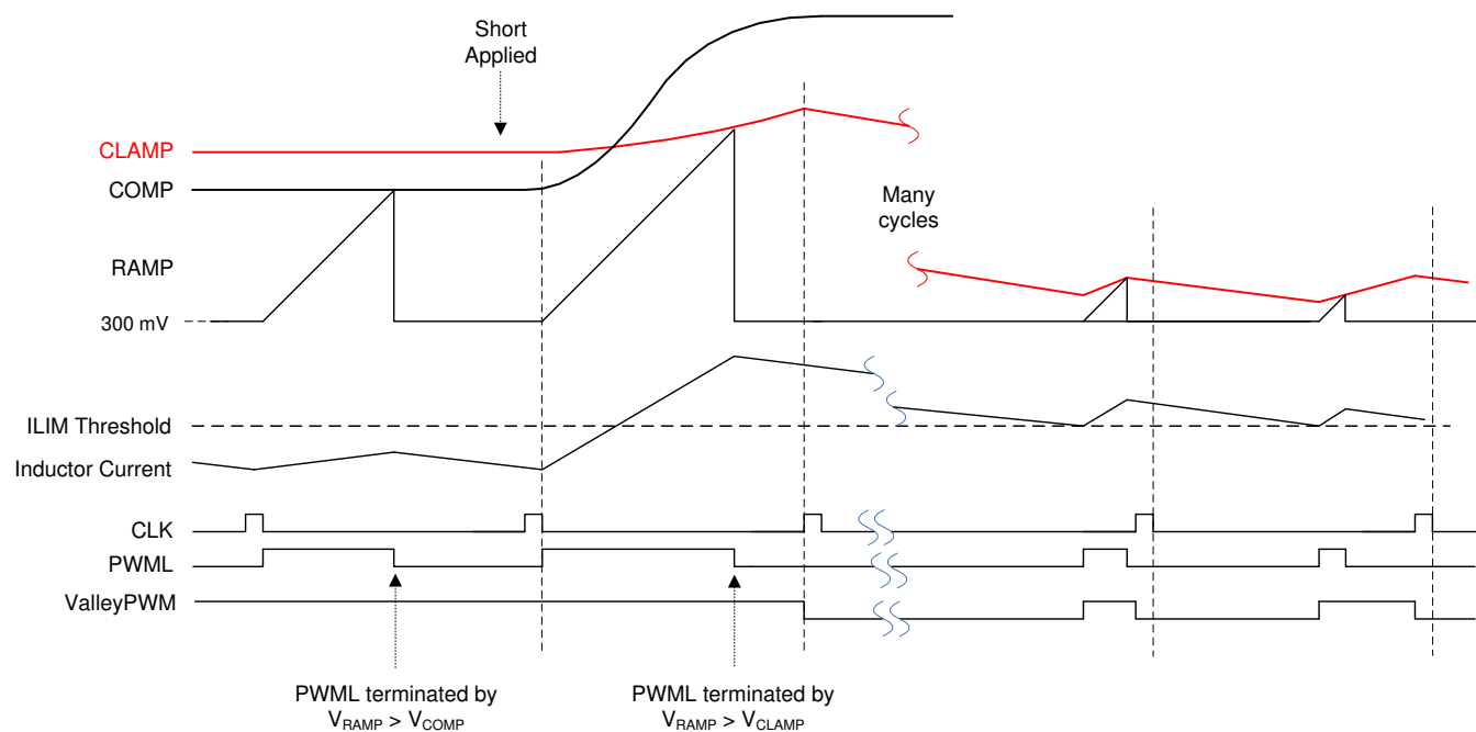
FIG 8-11. OCP Duty Cycle Limiting Waveforms
