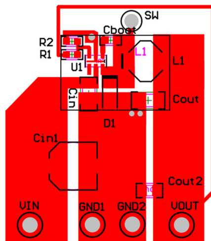
8-11. Layout Example
