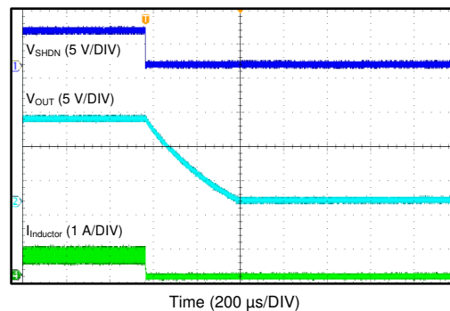
8-7. Shutdown Waveform
