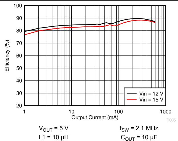
6-4. Efficiency versus Load Current
