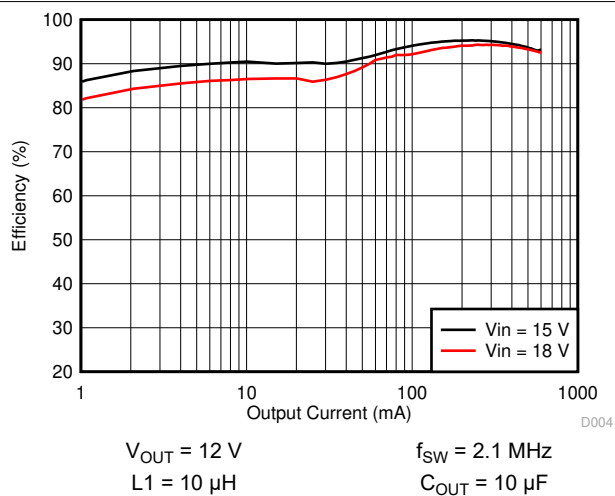
6-3. Efficiency versus Load Current
