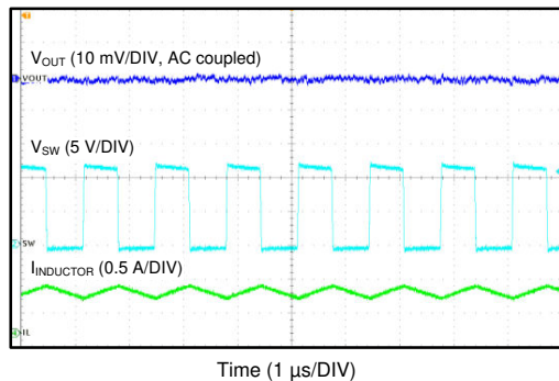
8-4. Switching Node and Output Voltage Waveform
