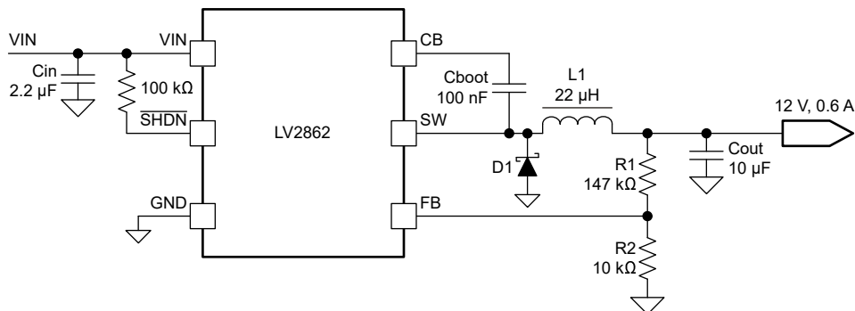
図 8-3. Application Circuit, 12-V Output
