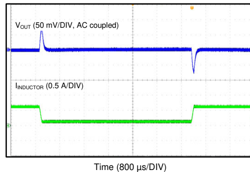
8-5. Load Transient Between 0.1 A and 0.6 A
