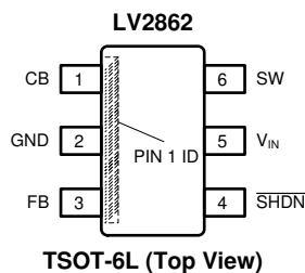
5-1. SOT (DDC) 6 Pins Top View
