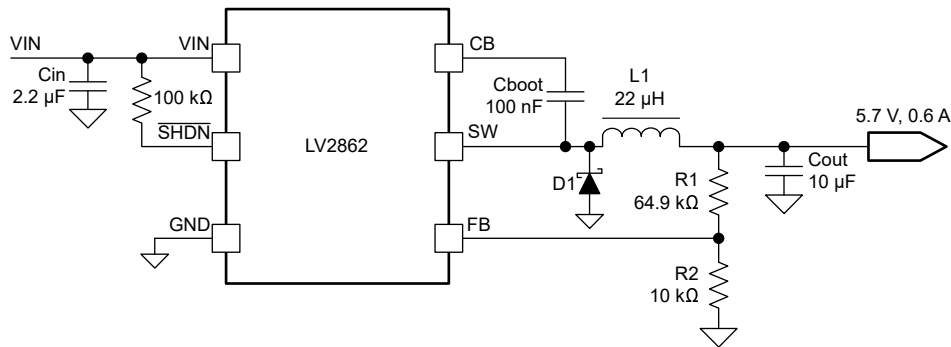
図 8-2. Application Circuit, 5.7-V Output
