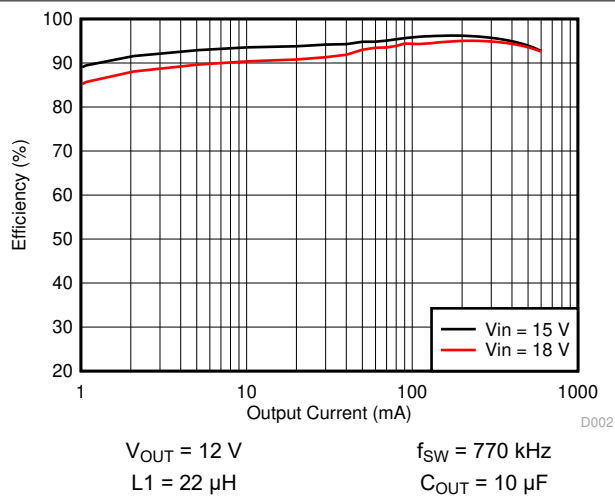
6-1. Efficiency versus Load Current
