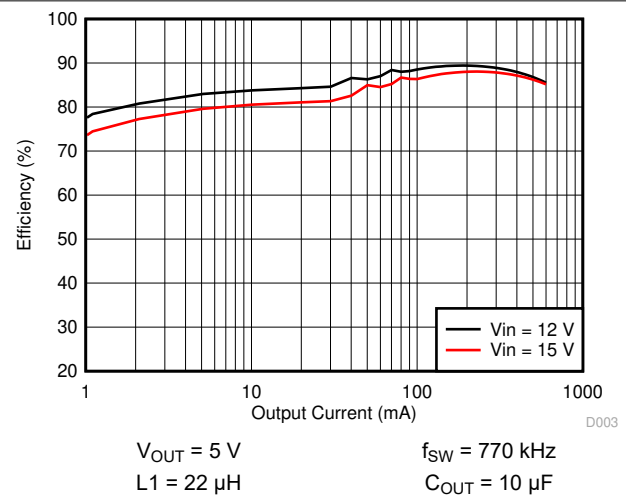
6-2. Efficiency versus Load Current
