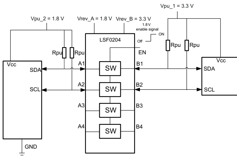
図 10-1. Bidirectional Translation to Multiple Voltage Levels
