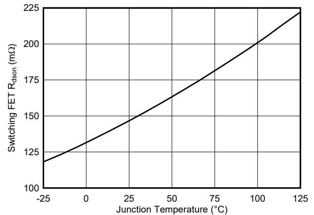
6-4. Switching FET R_{dson} vs. Junction Temperature
