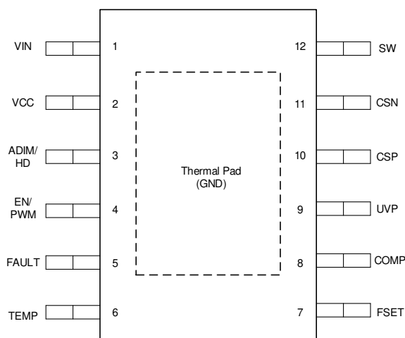
5-2. 12-Pin Buck HVSSOP Top View
