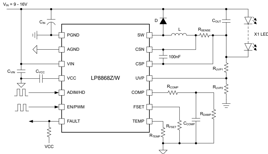
図 8-15. Typical Application for Buck Topology with LP8868Z
