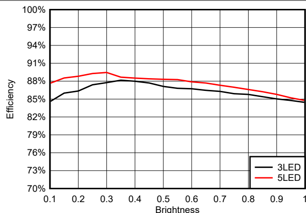
図 6-12. Efficiency at 1-A Max Output Current with Analogy Dimming, 22uH Inductor, Buck-Boost Topology
