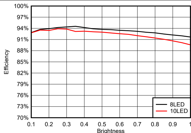
図 6-11. Efficiency at 1-A Max Output Current with Analogy Dimming, 22uH Inductor, Boost Topology
