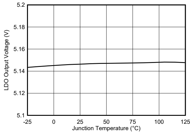
6-3. Internal LDO Output vs. Junction Temperature
