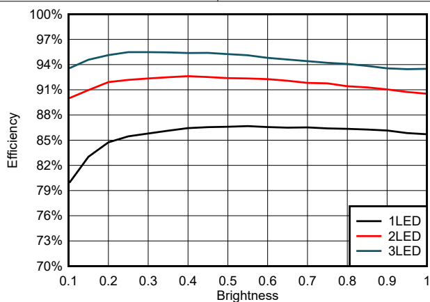
図 6-13. Efficiency at 3-A Max Output Current with Analogy Dimming, 22uH Inductor, Buck Topology
