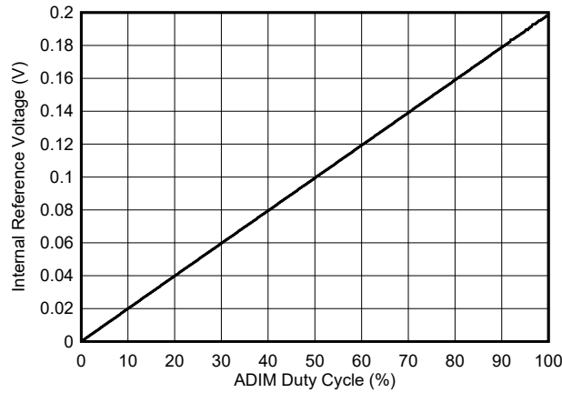
6-1. ADIM Duty Cycle vs. Reference Voltage in Analog Dimming
