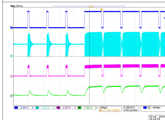
図 8-2. LED Current Ripple at ADIM = 100%, 1 kHz and F_{sw} = 400 kHz
