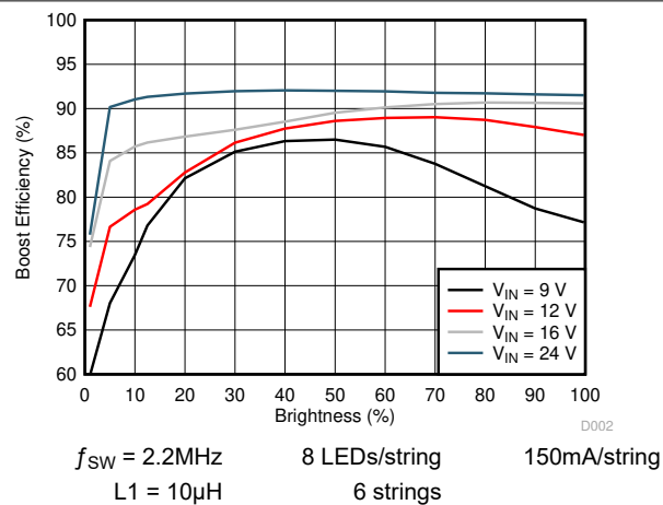
Figure 5-3. Boost Efficiency
