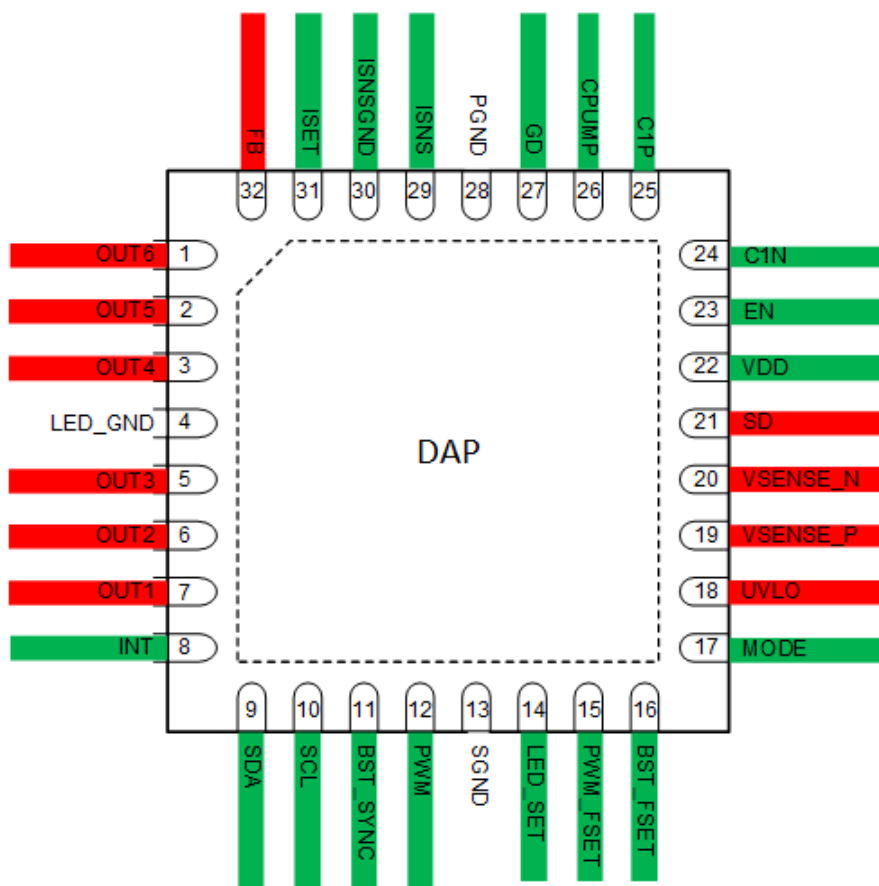
図 4-2. RHB Package 32-PIN QFN Top View
