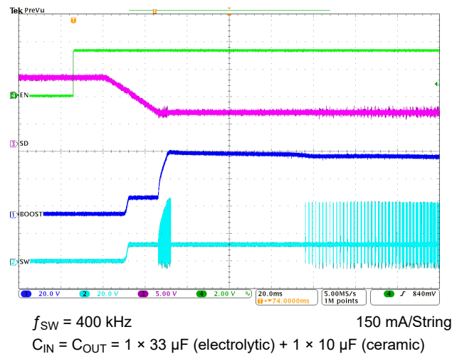
図 7-4. Typical Start-Up
