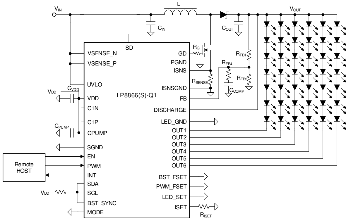
図 7-5. Minimal Solution/Minimum Components Application
