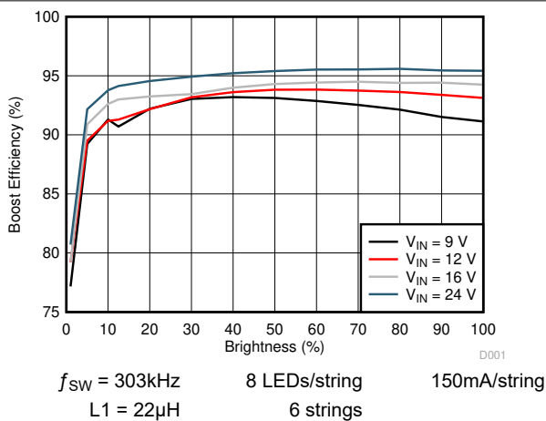
Figure 5-2. Boost Efficiency
