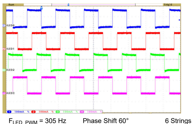
図 8-3. LED String Currents Showing Phase Shift PWM Operation
