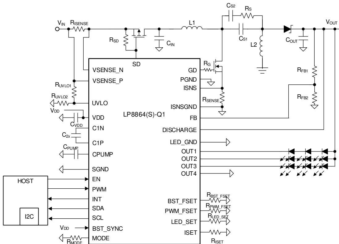
8-7. SEPIC Mode with Three LEDs in Series
