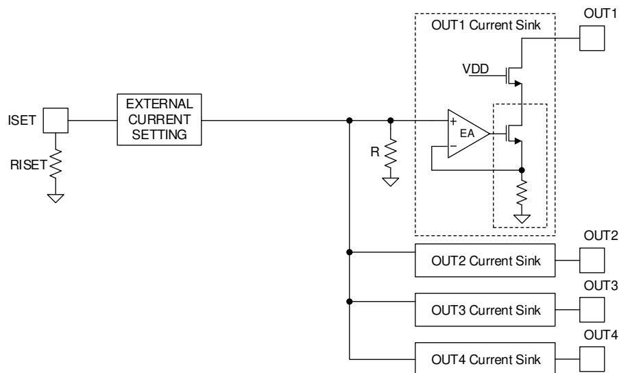
6-8. LED Driver Current Setting Circuit
