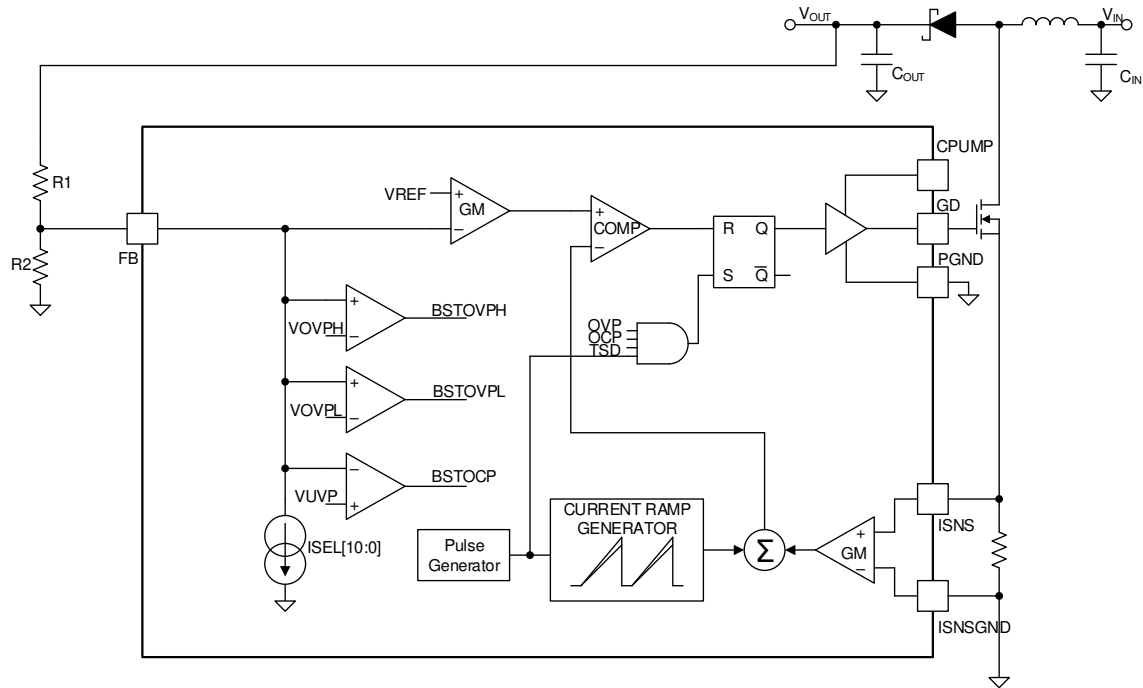
FIG 6-5. Two-Resistor FB Divider Circuit
