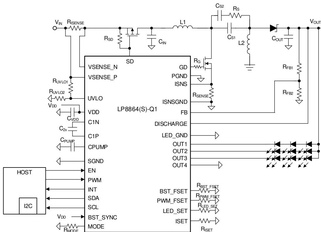
FIG 7-7. SEPIC Mode with Three LEDs in Series
