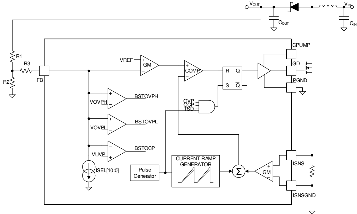
図 6-6. Three-Resistor FB Divider Circuit
